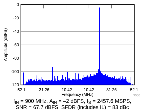
图 62. FFT in 24x Decimation (Complex Output)
