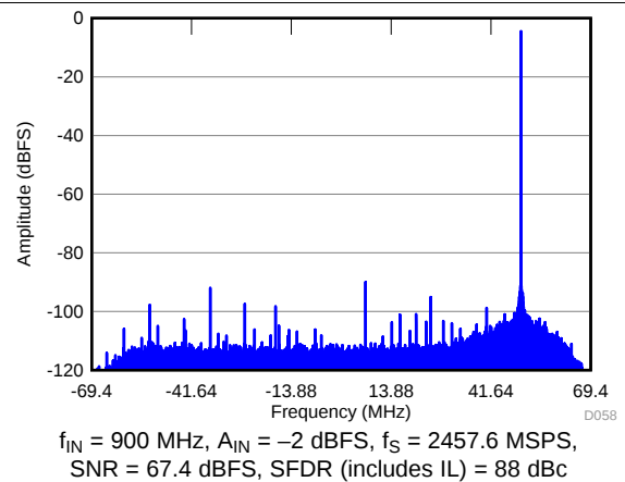
图 60. FFT in 18x Decimation (Complex Output)
