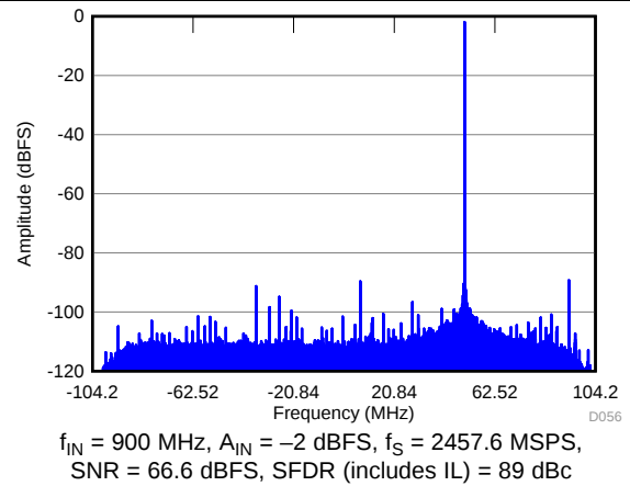
图 58. FFT in 12x Decimation (Complex Output)
