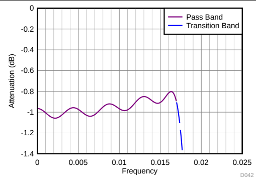
图 117. Divide-by-24 Filter Response (Zoomed)
