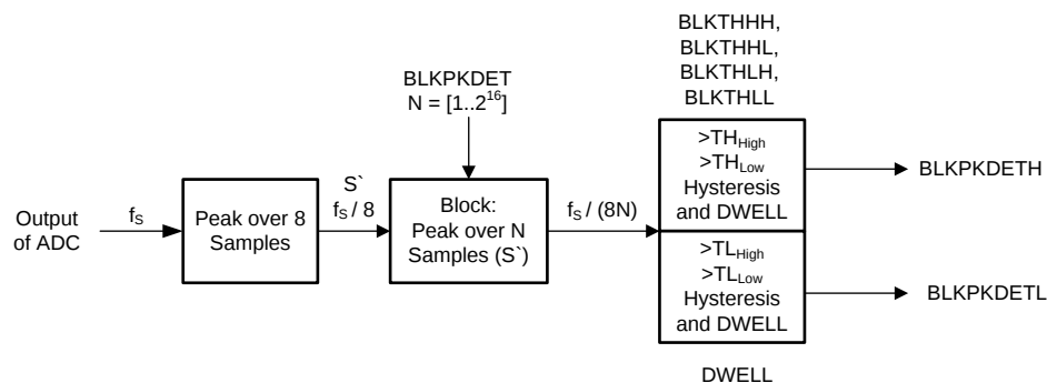
图 125. Peak Power Detector Implementation
