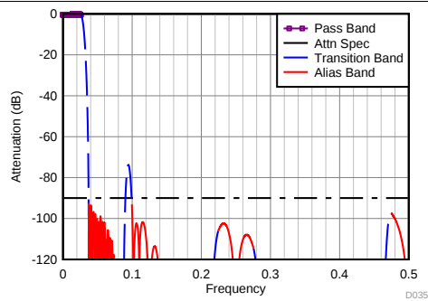
图 110. Divide-by-16 Filter Response
