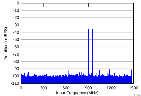
图 16. FFT for Two-Tone Input Signal (–36 dBFS)
