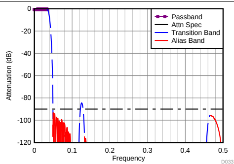
图 108. Divide-by-12 Filter Response
