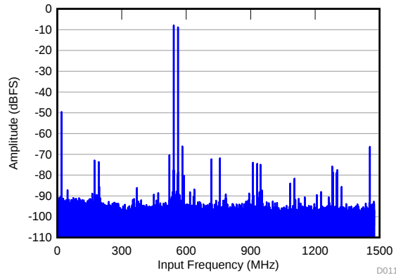
图 27. FFT for Two-Tone Input Signal (–8 dBFS)
