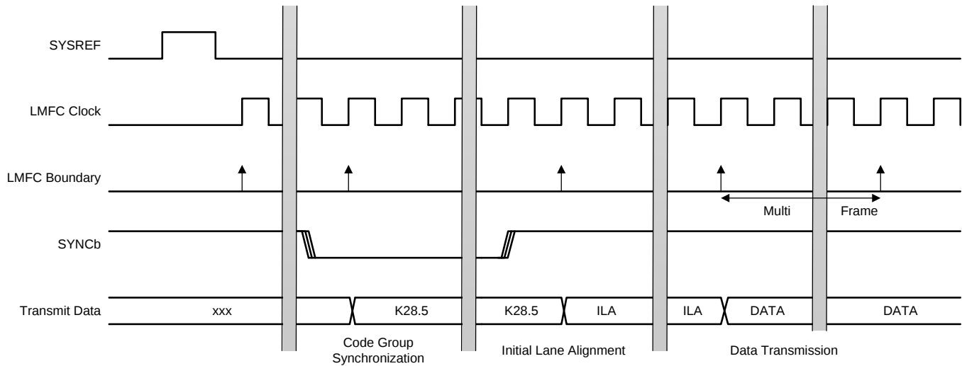
图 134. JESD Internal Timing Information
