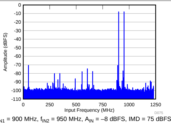
图 15. FFT for Two-Tone Input Signal (–8 dBFS)
