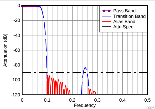
图 100. Divide-by-6 Filter Response
