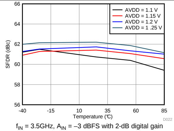
图 46. Spurious-Free Dynamic Range vs AVDD Supply and Temperature
