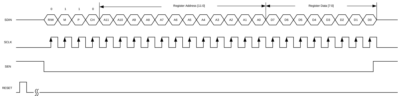
图 140. SPI Write Timing Diagram for Digital Bank Register Write
