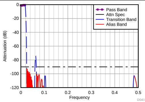
图 116. Divide-by-24 Filter Response
