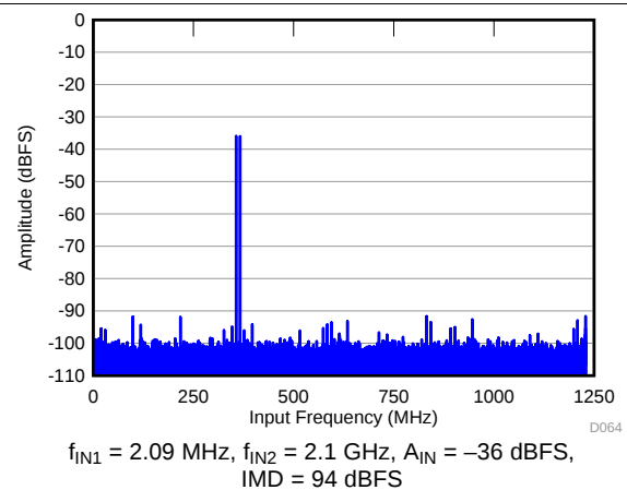
图 26. FFT for Two-Tone Input Signal (–36 dBFS, f_s = 2457.6 \text{ MSPS} )
