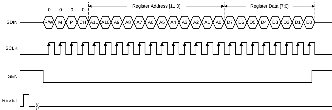
图 137. SPI Write Timing Diagram for the Analog Bank
