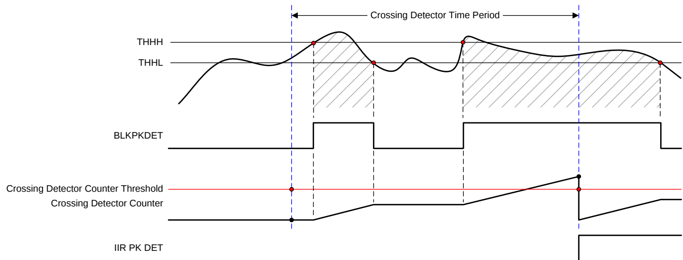
图 128. Crossing Detector Timing Diagram
