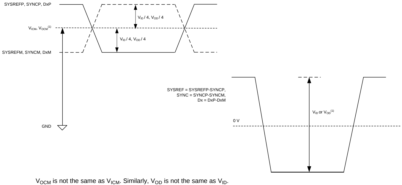
图 1. Logic Levels for Digital Inputs and Outputs
