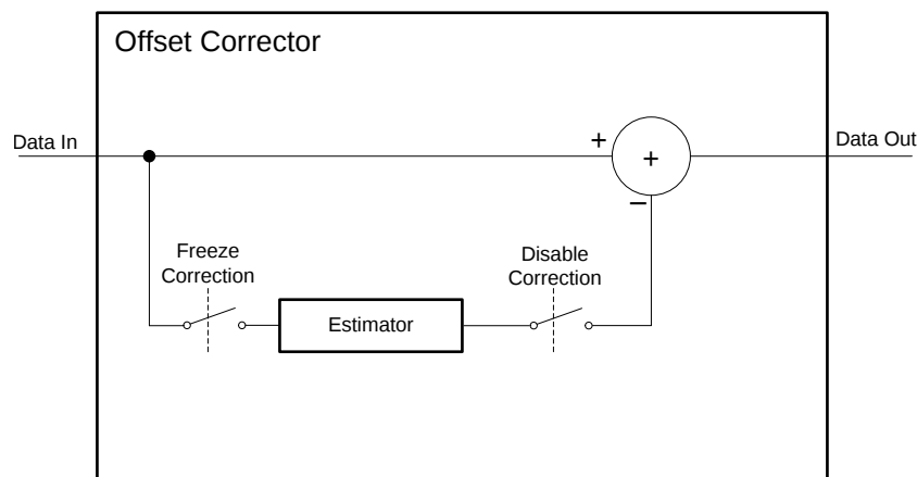
图 258. Offset Corrector in the ADC32RF8x
