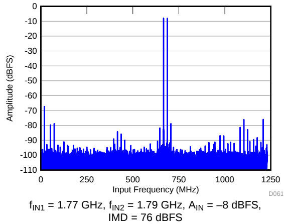
图 21. FFT for Two-Tone Input Signal (–8 dBFS, f_s = 2457.6 \text{ MSPS} )
