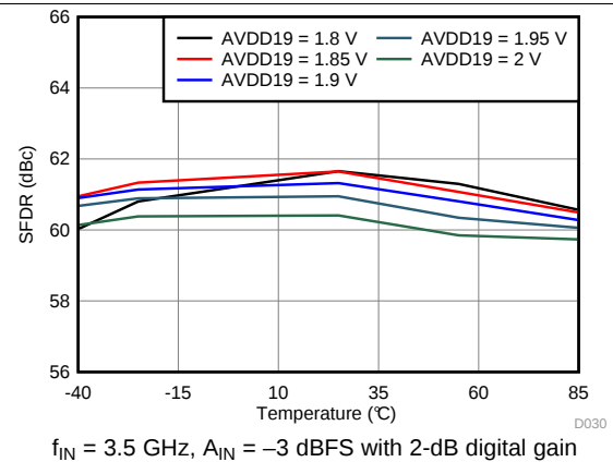
图 54. Spurious-Free Dynamic Range vs AVDD19 Supply and Temperature
