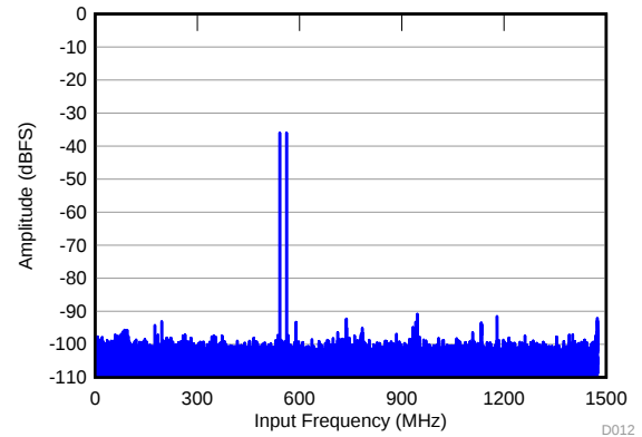
图 28. FFT for Two-Tone Input Signal (–36 dBFS)
