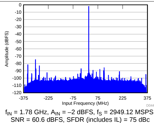
图 68. FFT in 4X Decimation (Complex Output)
