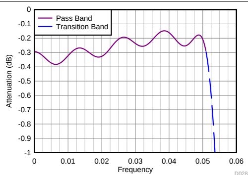
图 103. Divide-by-8 Filter Response (Zoomed)
