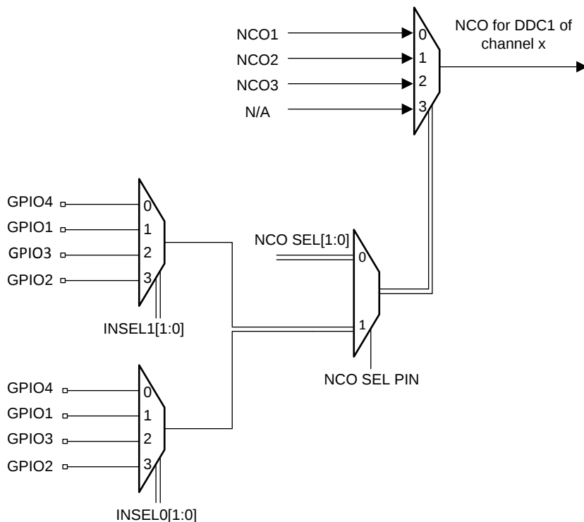
图 121. NCO Switching from GPIO and SPI
