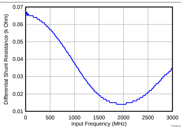
图 83. Differential Input Resistance vs Input Frequency
