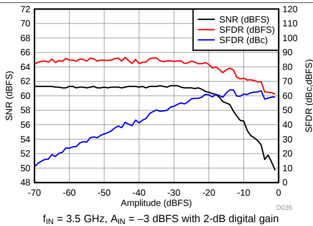
图 59. Performance vs Amplitude
