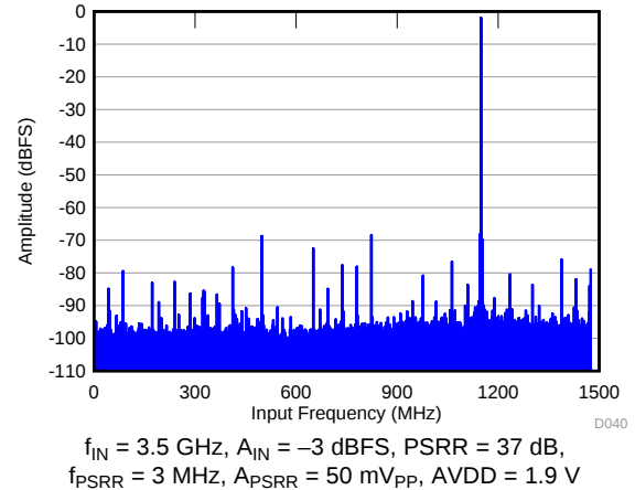
图 64. Power-Supply Rejection Ratio FFT for Test Signal on AVDD Supply
