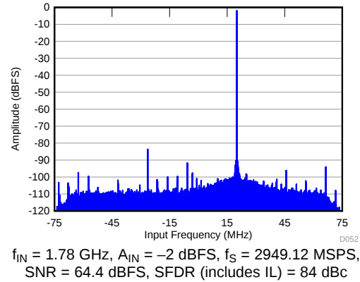
图 76. FFT in 20X Decimation (Complex Output)
