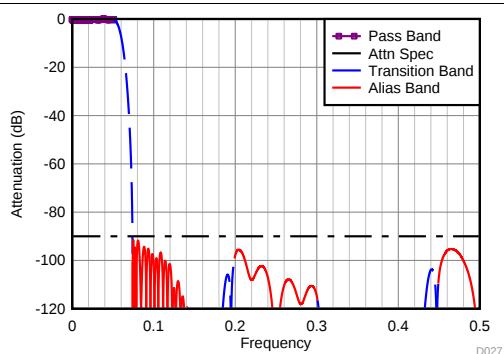
图 102. Divide-by-8 Filter Response
