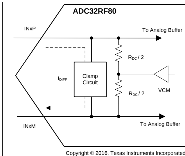
图 85. Clamp Circuit in the ADC32RF8x
