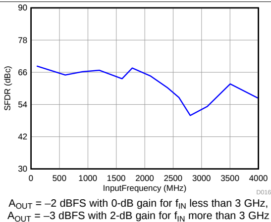
图 37. Spurious-Free Dynamic Range vs Input Frequency
