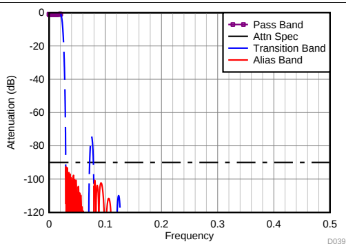
图 114. Divide-by-20 Filter Response
