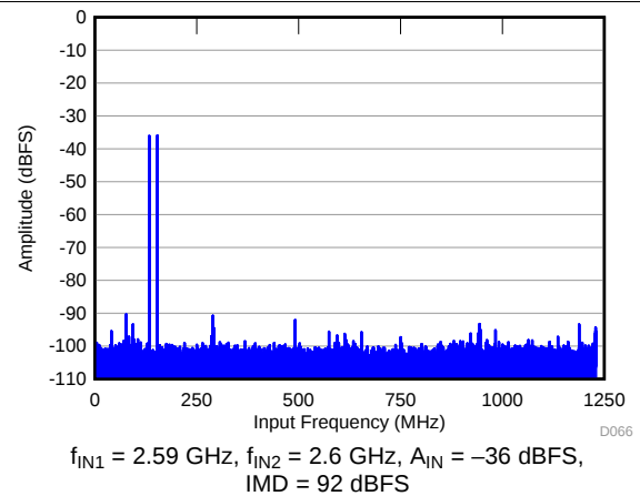
图 30. FFT for Two-Tone Input Signal (–36 dBFS, f_s = 2457.6 \text{ MSPS} )
