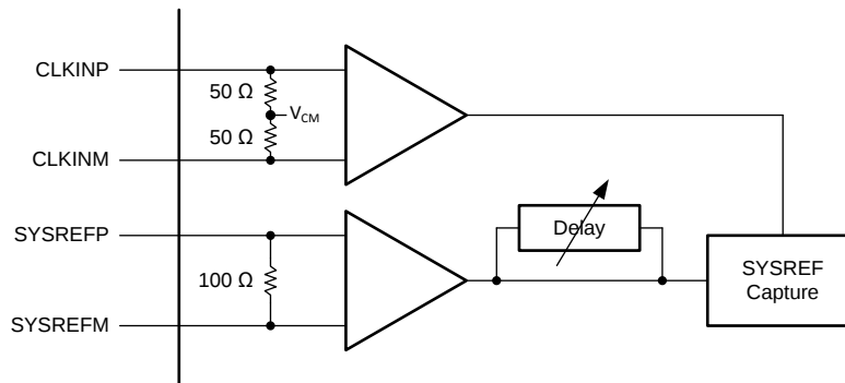
图 89. SYSREF Internal Circuit Diagram
