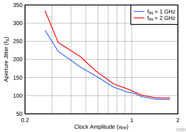
图 88. Equivalent Aperture Jitter vs Input Clock Amplitude
