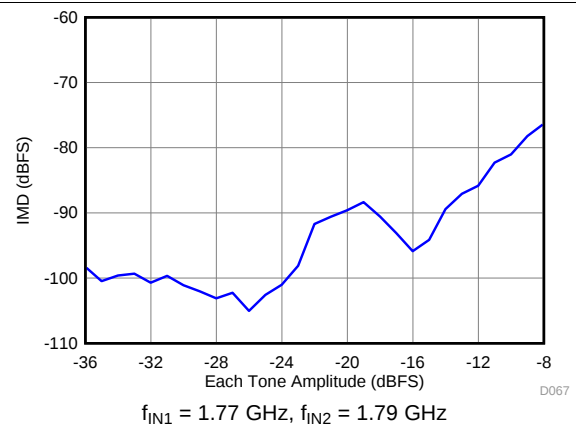
图 32. Intermodulation Distortion vs Input Amplitude (1770 MHz and 1790 MHz, f_s = 2457.6 \text{ MSPS} )
