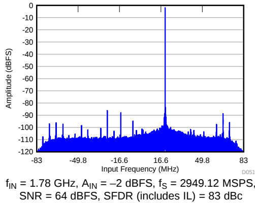
图 75. FFT in 18X Decimation (Complex Output)
