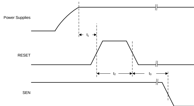
图 253. Hardware Reset Timing Diagram
