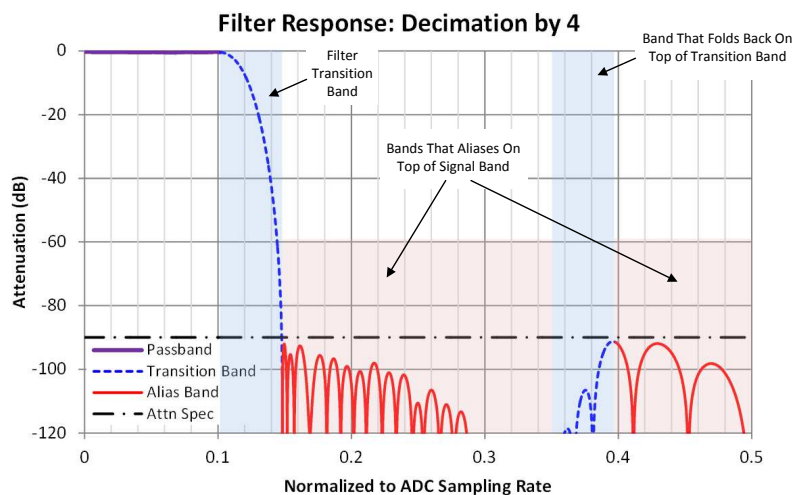
图 97. Interpretation of the Decimation Filter Plots
