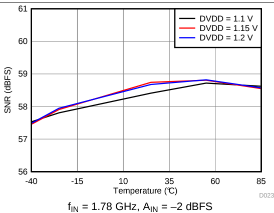
图 47. Signal-to-Noise Ratio vs DVDD Supply and Temperature
