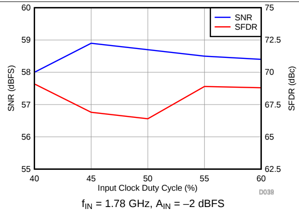
图 62. Performance vs Clock Duty Cycle
