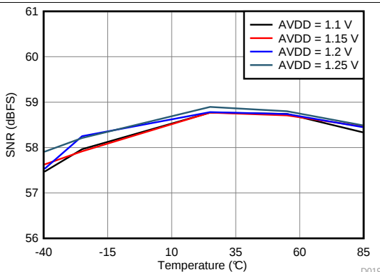
图 43. Signal-to-Noise Ratio vs AVDD Supply and Temperature
