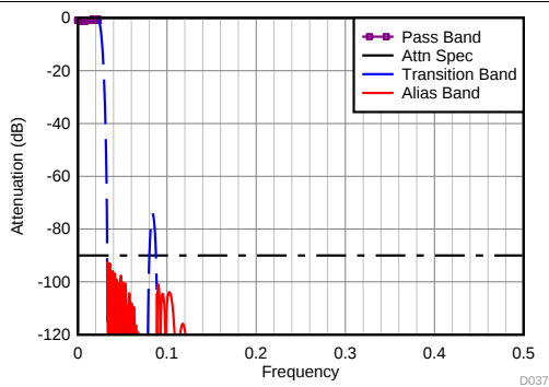
图 112. Divide-by-18 Filter Response
