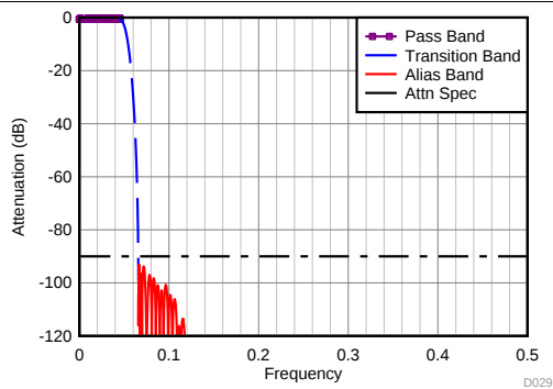
图 104. Divide-by-9 Filter Response
