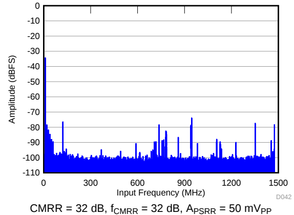
图 66. Common-Mode Rejection Ratio FFT
