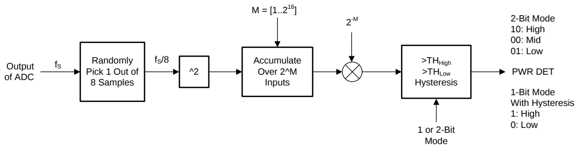
图 129. RMS Power Detector Implementation
