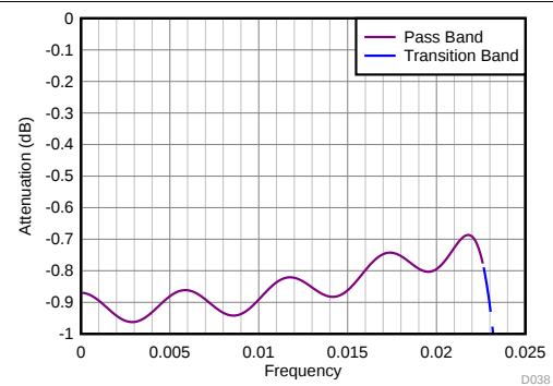
图 113. Divide-by-18 Filter Response (Zoomed)
