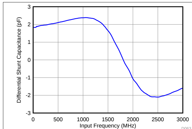
图 82. Differential Input Capacitance vs Input Frequency
