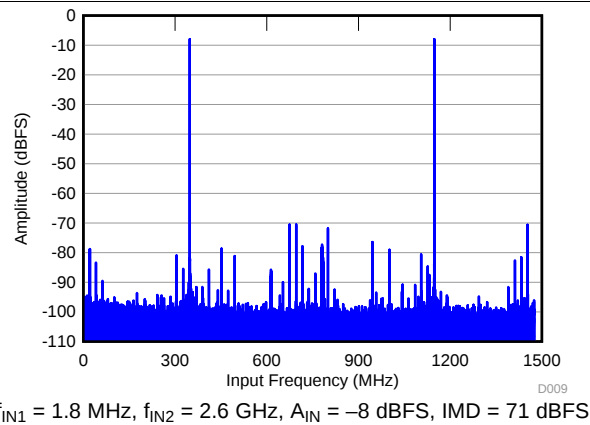
图 23. FFT for Two-Tone Input Signal (–8 dBFS)
