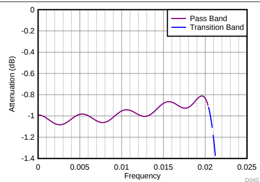
图 115. Divide-by-20 Filter Response (Zoomed)
