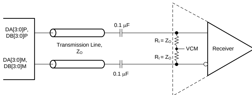
图 122. External Serial JESD204B Interface Connection
