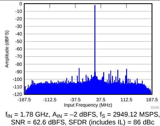
图 70. FFT in 8X Decimation (Complex Output)
