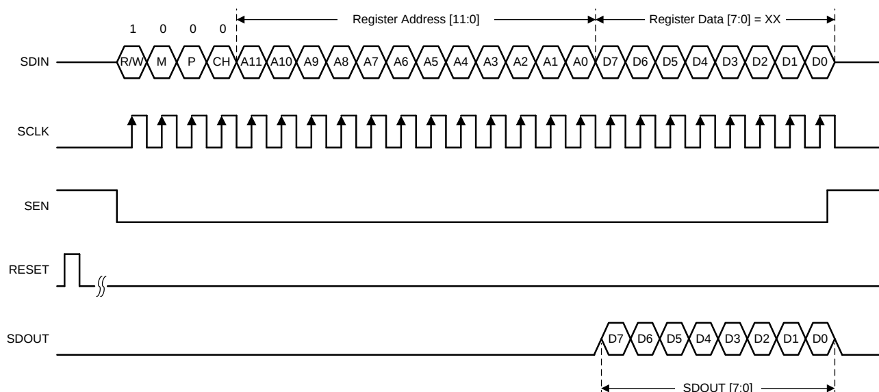
图 138. SPI Read Timing Diagram for the Analog Bank
