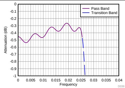
图 111. Divide-by-16 Filter Response (Zoomed)
