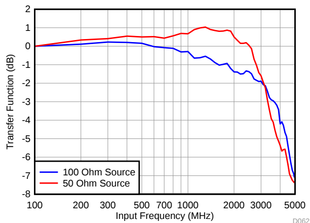
图 84. Input Bandwidth with a 100-Ω Source Resistance
