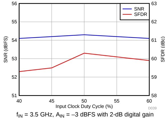
图 63. Performance vs Clock Duty Cycle
