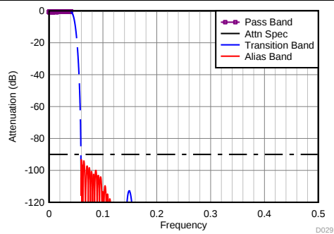
图 106. Divide-by-10 Filter Response
