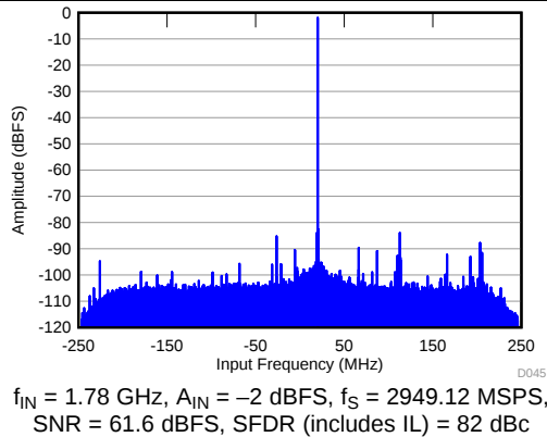
图 69. FFT in 6X Decimation (Complex Output)
