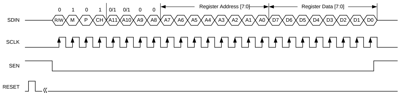
图 142. SPI Write Timing Diagram for the Decimation and Power Detector Pages
