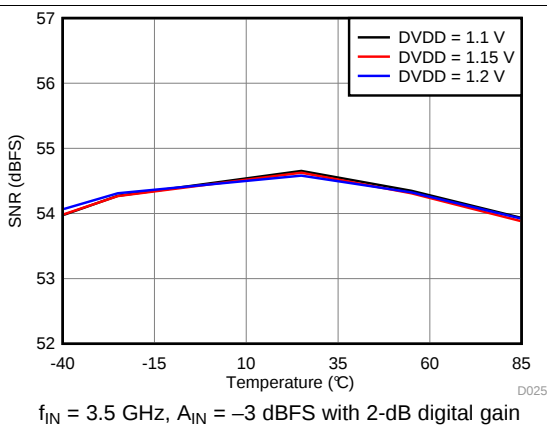
图 49. Signal-to-Noise Ratio vs DVDD Supply and Temperature
