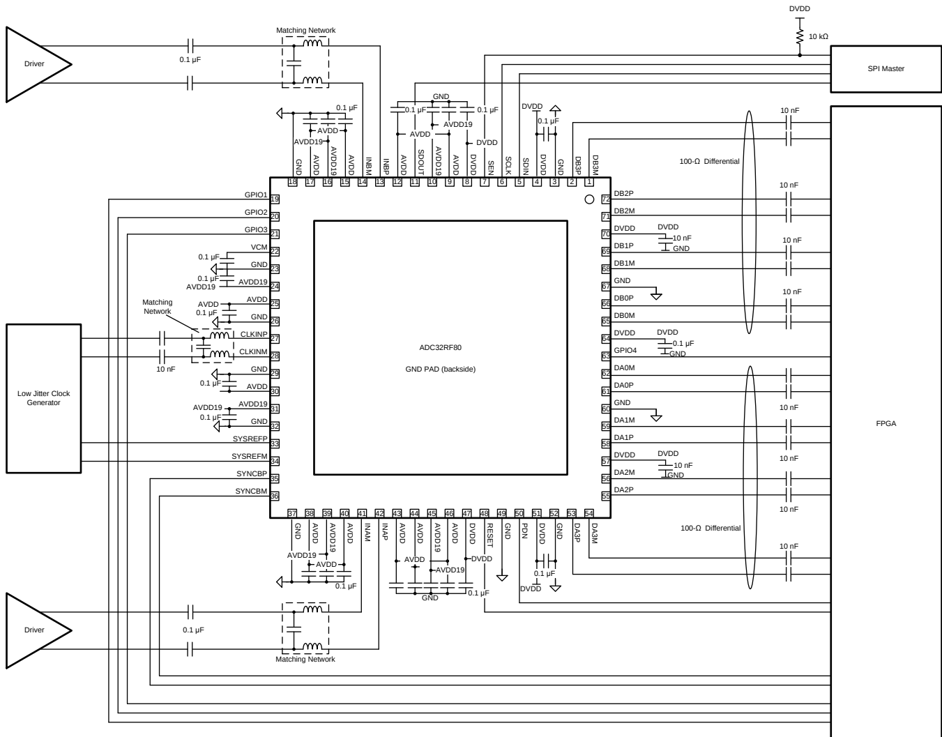
图 261. Typical Application Implementation Diagram
