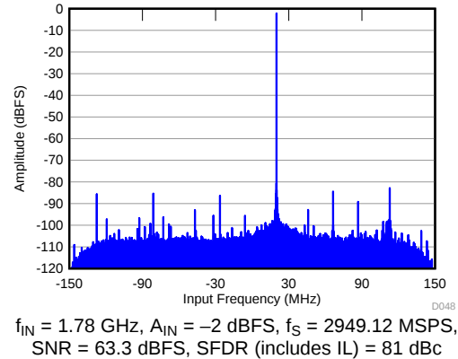
图 72. FFT in 10X Decimation (Complex Output)
