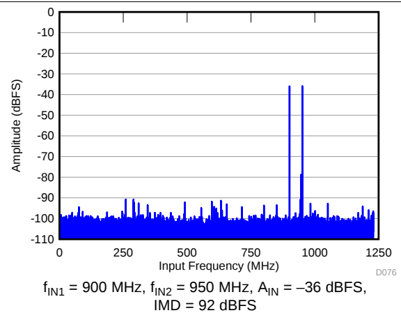
图 18. FFT for Two-Tone Input Signal (–36 dBFS, f_s = 2457.6 \text{ MSPS} )
