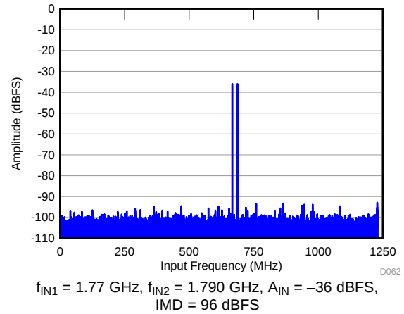
图 22. FFT for Two-Tone Input Signal (–36 dBFS, f_s = 2457.6 \text{ MSPS} )
