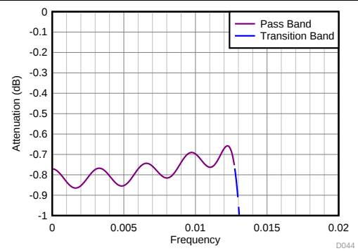
图 119. Divide-by-32 Filter Response (Zoomed)
