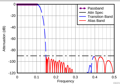
图 98. Divide-by-4 Filter Response
