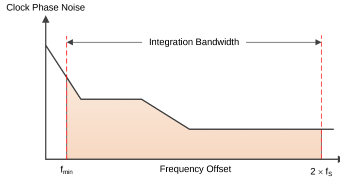
图 255. Integration Bandwidth for Extracting Jitter from Clock Phase Noise
