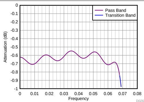
图 101. Divide-by-6 Filter Response (Zoomed)
