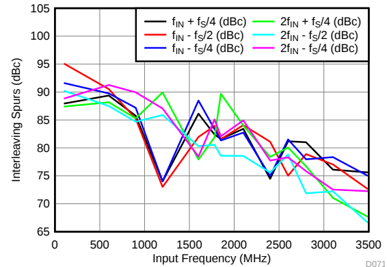
图 40. IL Spur vs Input Frequency ( f_S = 2457.6 MSPS)
