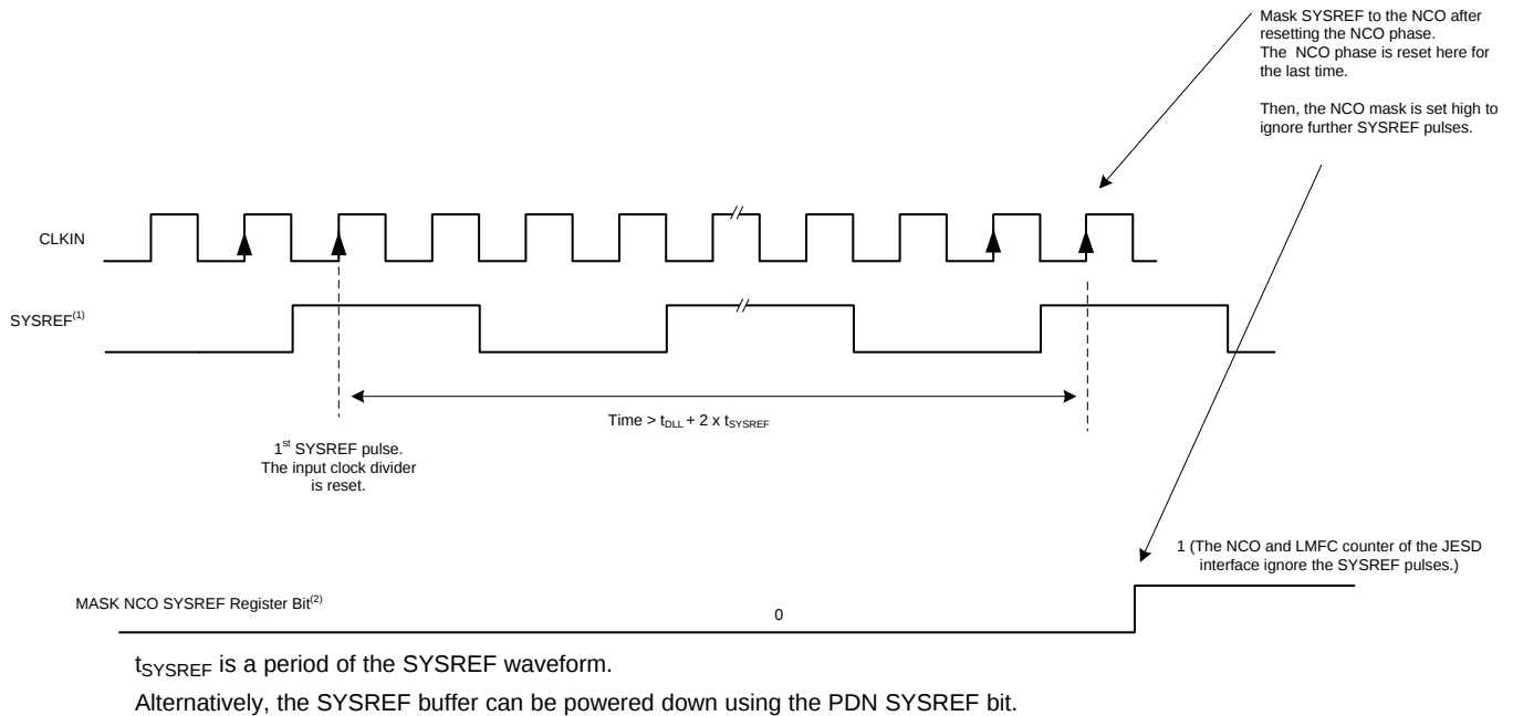
图 92. SYSREF Used as a Periodic Waveform
