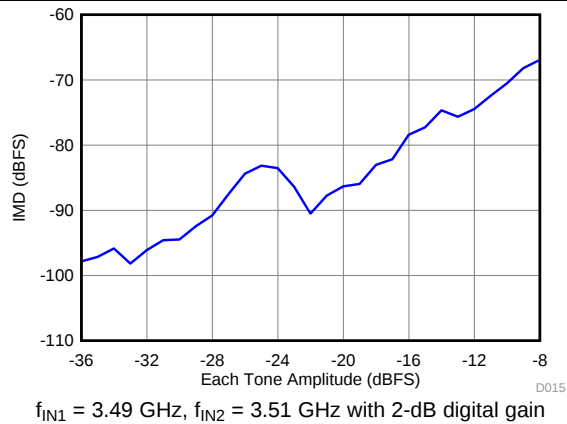
图 35. Intermodulation Distortion vs Input Amplitude (3490 MHz and 3510 MHz)
