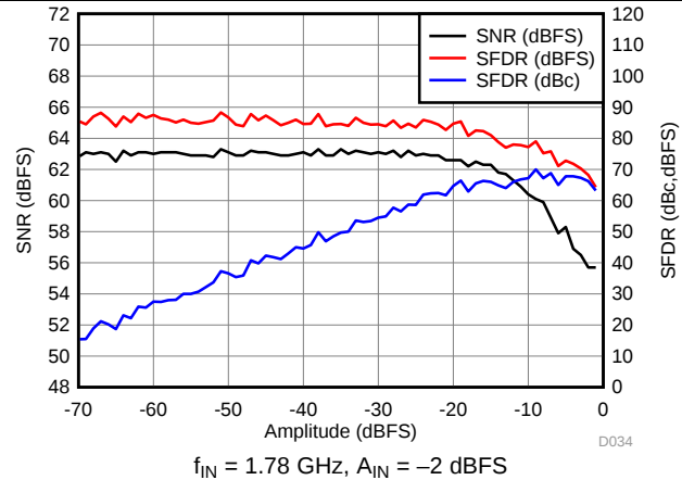
图 58. Performance vs Amplitude
