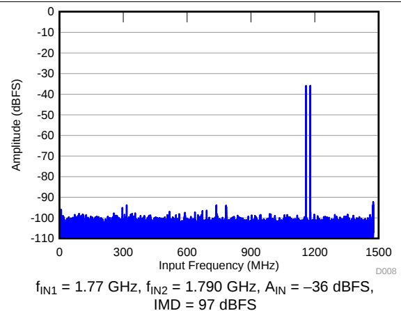
图 20. FFT for Two-Tone Input Signal (–36 dBFS)
