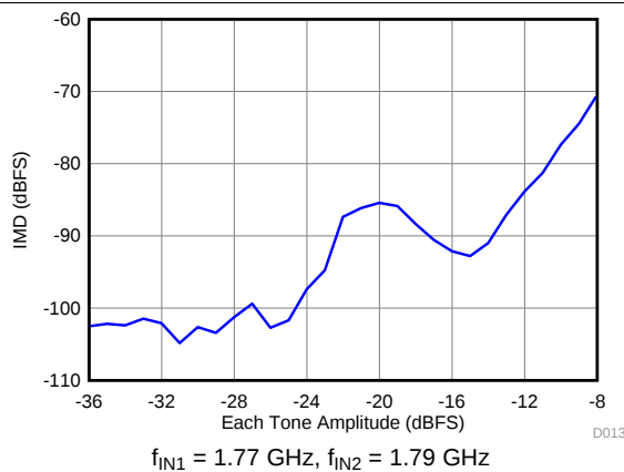
图 31. Intermodulation Distortion vs Input Amplitude (1770 MHz and 1790 MHz)
