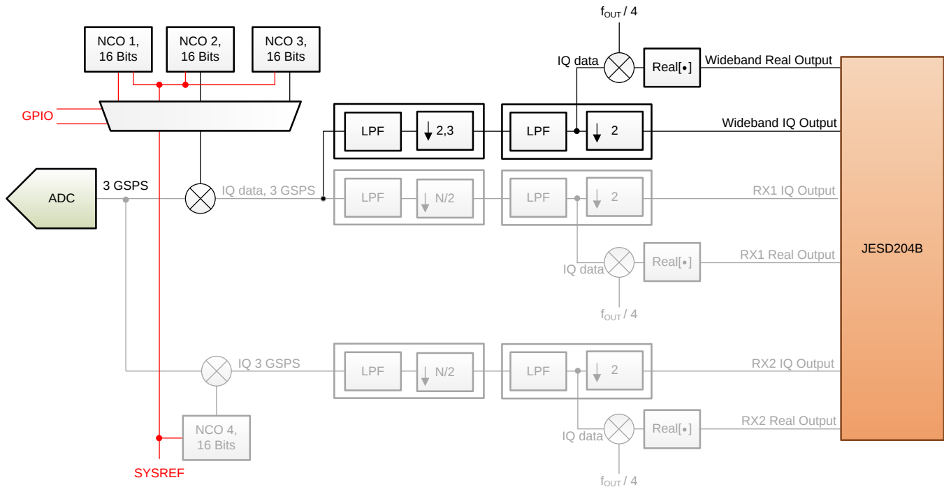
图 95. Decimation Filter Implementation for Single-Band and Wide-Bandwidth Mode
