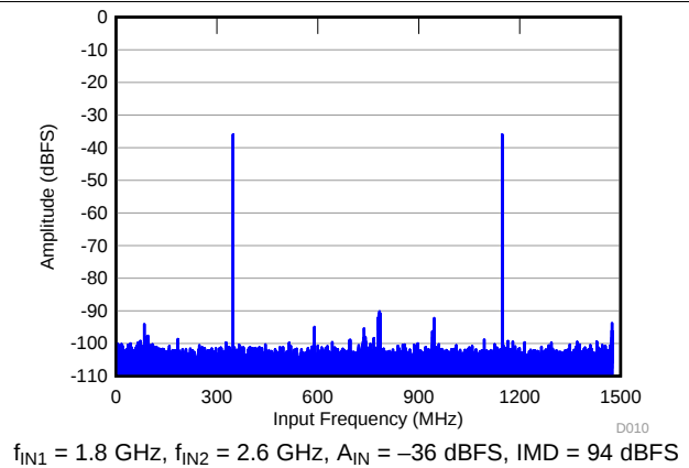
图 24. FFT for Two-Tone Input Signal
