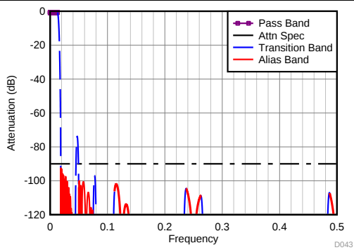
图 118. Divide-by-32 Filter Response
