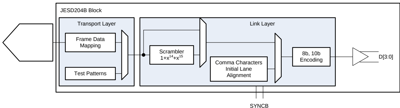
图 133. JESD Digital Block Implementation
