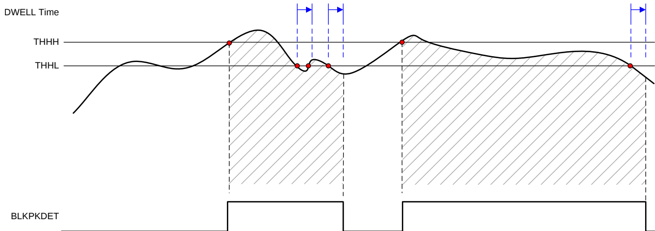
图 126. Peak Power Detector Timing Diagram
