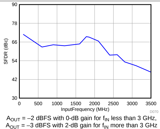
图 38. Spurious-Free Dynamic Range vs Input Frequency ( f_s = 2457.6 \text{ MSPS} )
