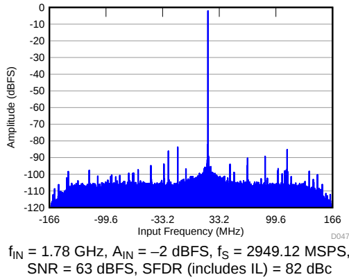
图 71. FFT in 9X Decimation (Complex Output)
