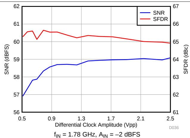
图 60. Performance vs Clock Amplitude
