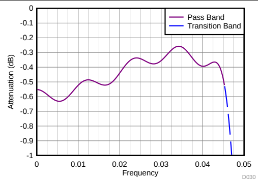
图 105. Divide-by-9 Filter Response (Zoomed)
