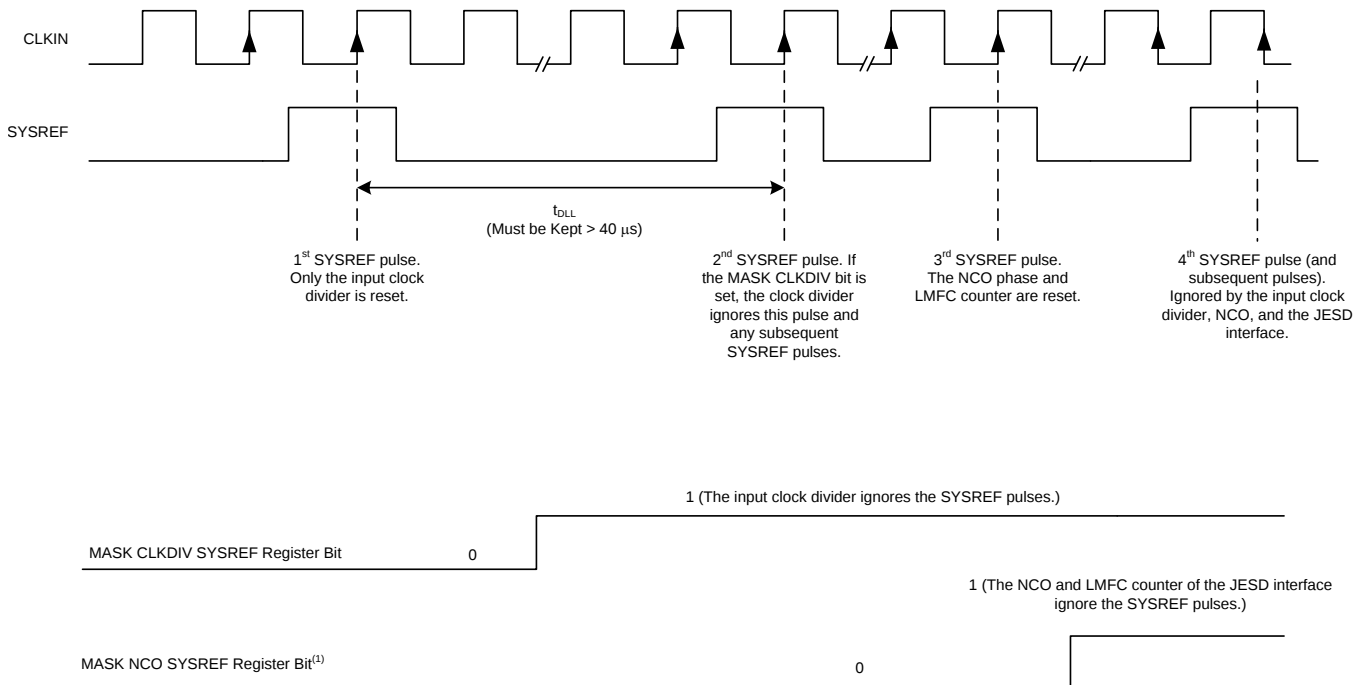
图 91. SYSREF Used as a Periodic, Finite Number of Pulses
