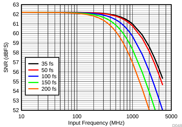
图 254. ADC SNR vs Input Frequency and External Clock Jitter
