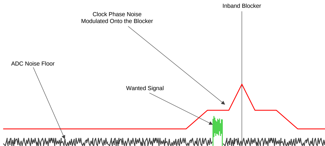
图 256. Small Wanted Signal in Presence of Interferer
