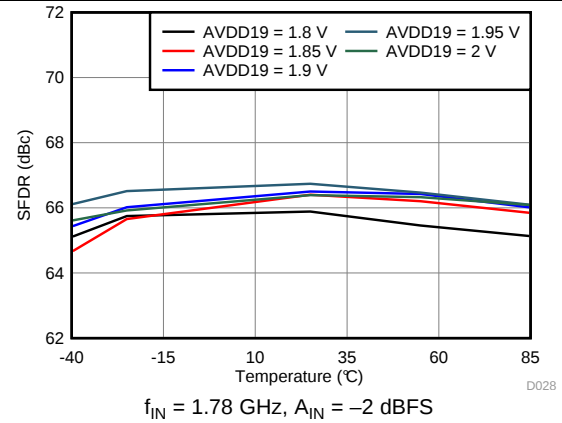
图 52. Spurious-Free Dynamic Range vs AVDD19 Supply and Temperature
