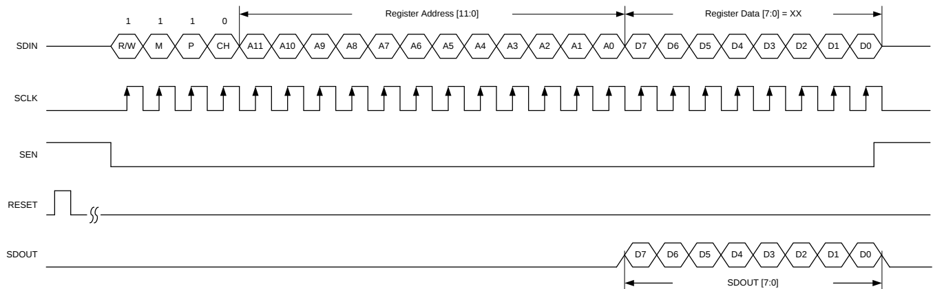
图 141. SPI Read Timing Diagram for the Digital Bank
