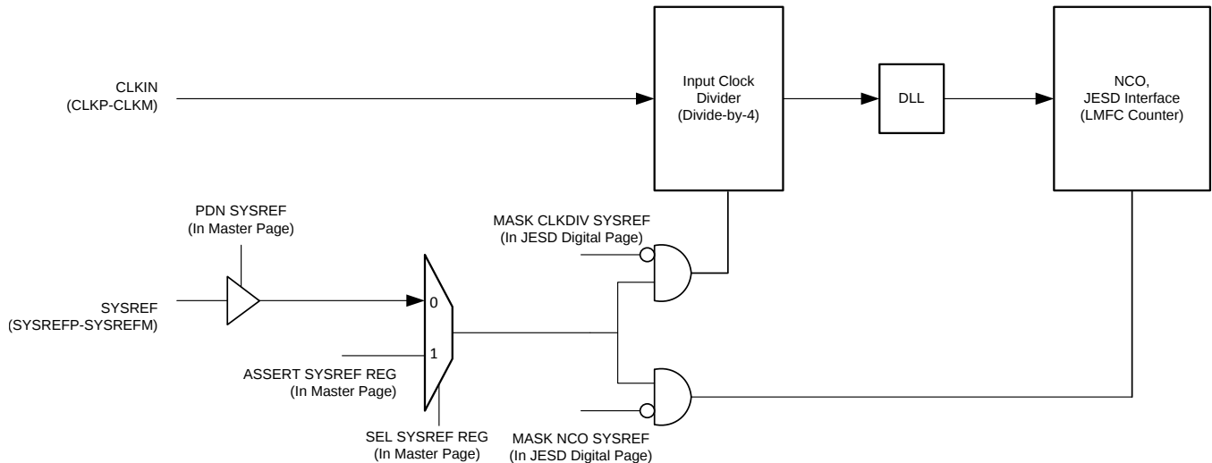
图 90. Using SYSREF to Reset the Clock Divider, the NCO, and the LMFC Counter
