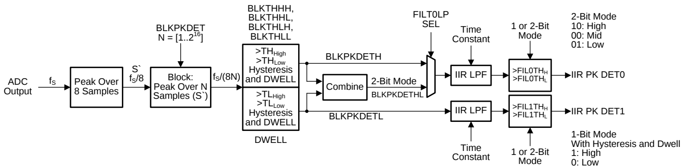
图 127. Crossing Detector Implementation
