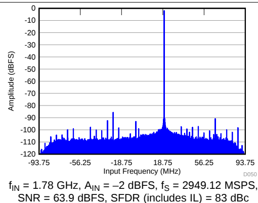
图 74. FFT in 16X Decimation (Complex Output)
