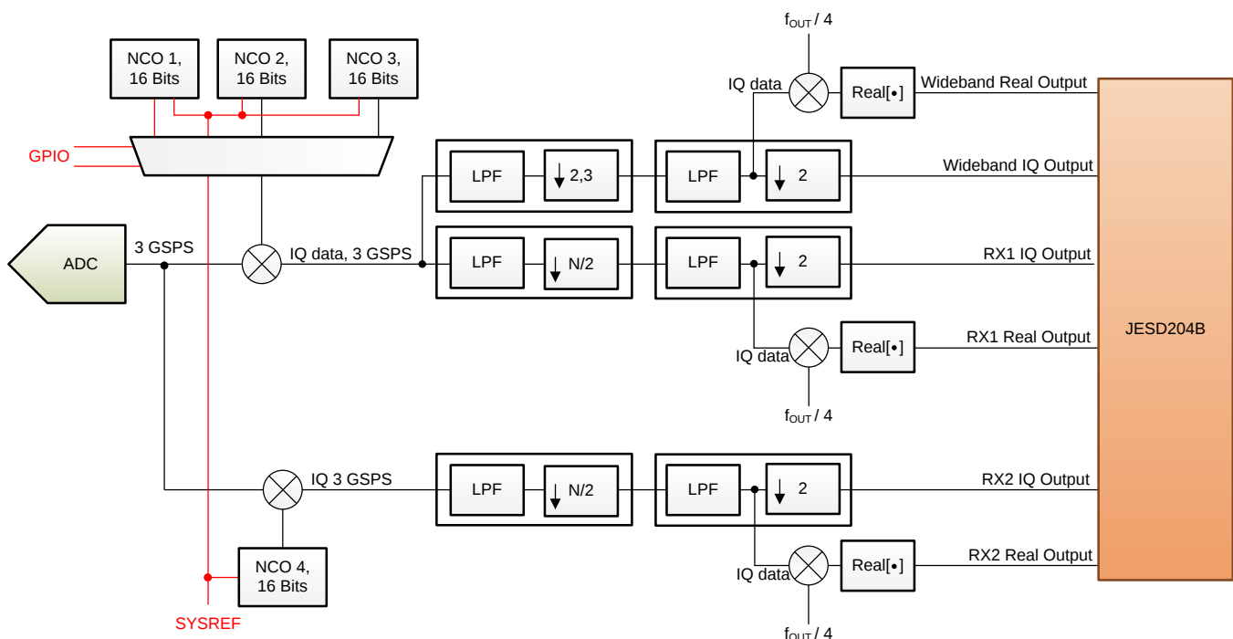
图 93. DDC Chains Overview (One ADC Channel Shown)
