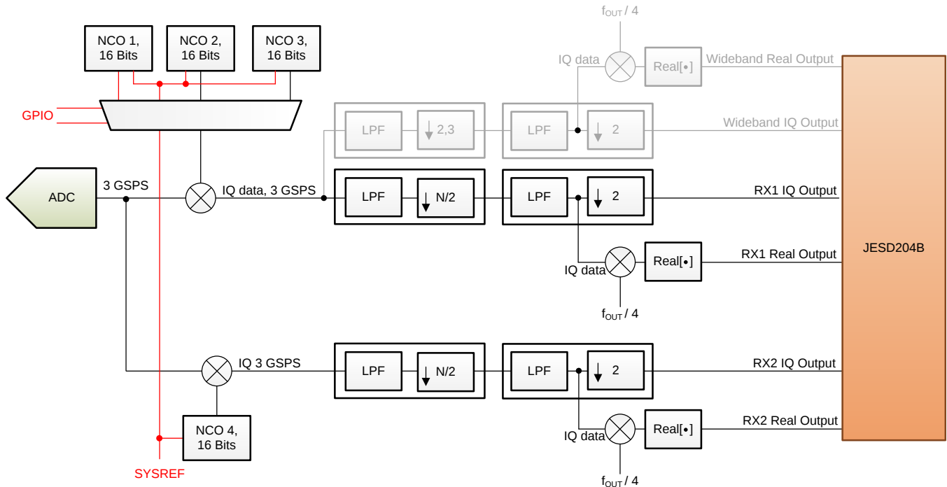
图 94. Decimation Filter Option for Single- or Dual-Band Operation
