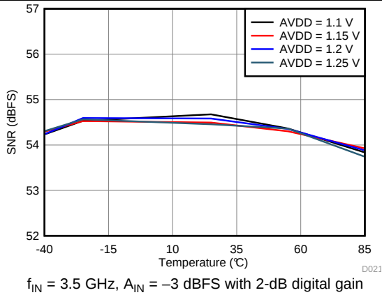
图 45. Signal-to-Noise Ratio vs AVDD Supply and Temperature
