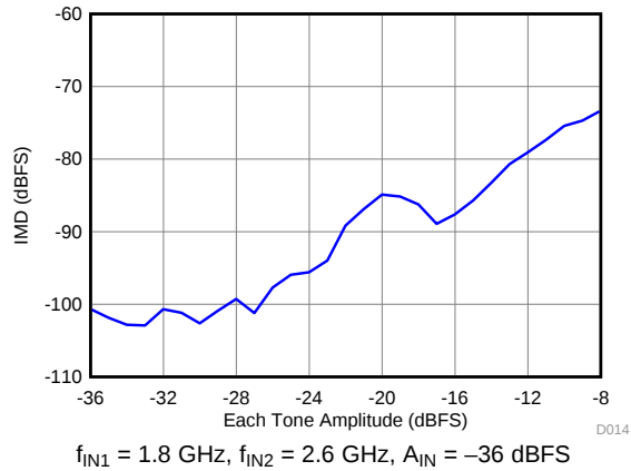
图 33. Intermodulation Distortion vs Input Amplitude (1800 MHz and 2600 MHz)
