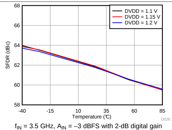
图 50. Spurious-Free Dynamic Range vs DVDD Supply and Temperature
