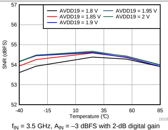
图 53. Signal-to-Noise Ratio vs AVDD19 Supply and Temperature
