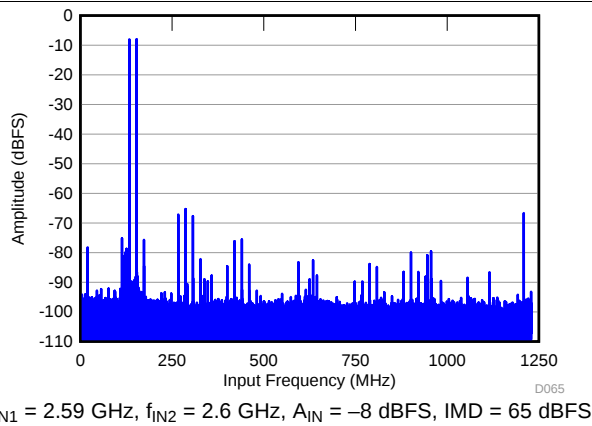
图 27. FFT for Two-Tone Input Signal (–8 dBFS)
