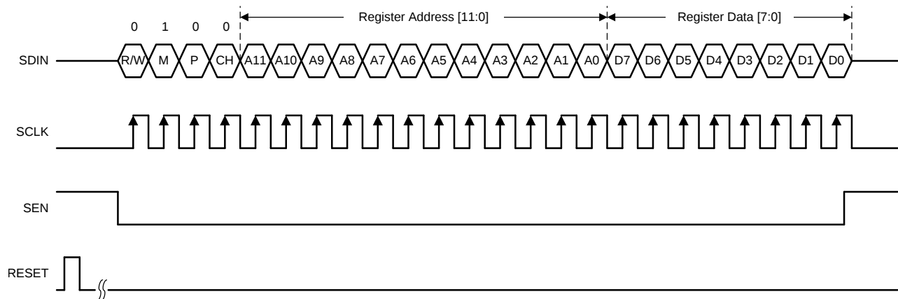
图 139. SPI Write Timing Diagram for Digital Bank Page Selection
