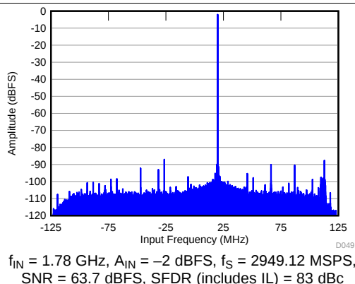
图 73. FFT in 12X Decimation (Complex Output)
