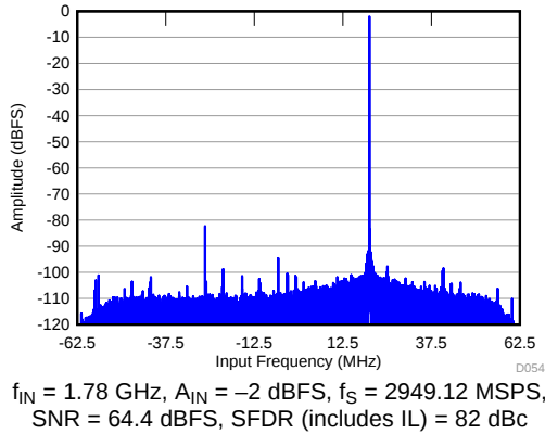
图 77. FFT in 24X Decimation (Complex Output)
