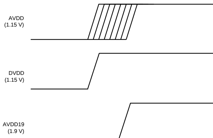
图 265. Power Sequencing for the ADC32RF8x Family of devices
