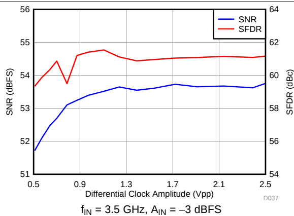
图 61. Performance vs Clock Amplitude
