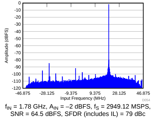
图 78. FFT in 32X Decimation (Complex Output)
