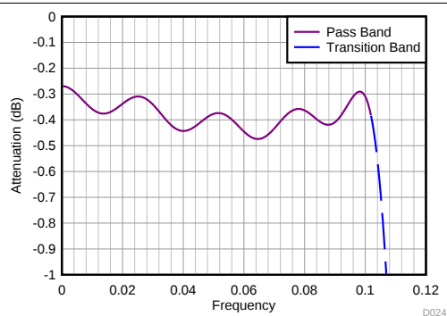
图 99. Divide-by-4 Filter Response (Zoomed)
