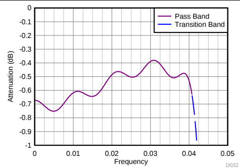
图 107. Divide-by-10 Filter Response (Zoomed)
