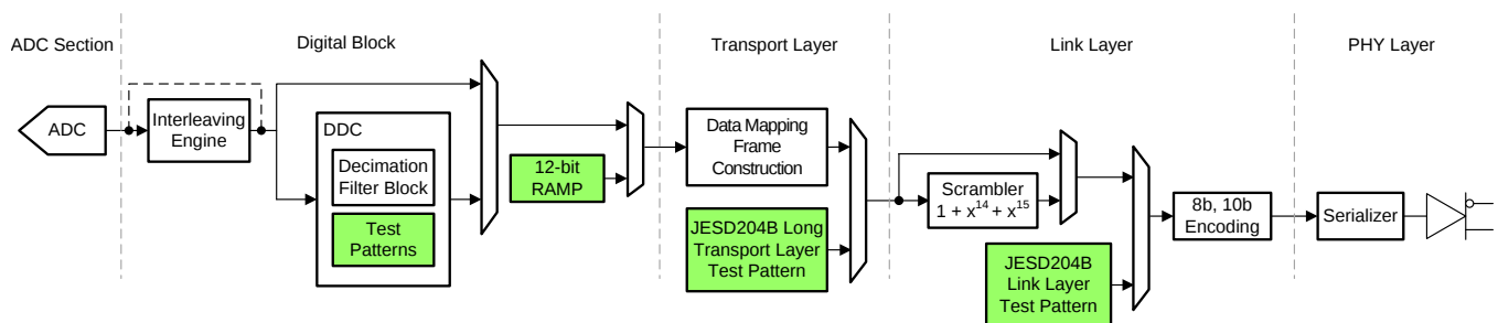
图 131. Test Pattern Generator Implementation
