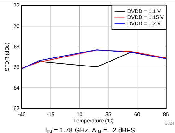
图 48. Spurious-Free Dynamic Range vs DVDD Supply and Temperature
