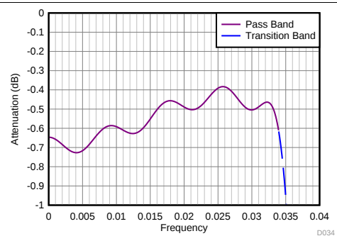
图 109. Divide-by-12 Filter Response (Zoomed)
