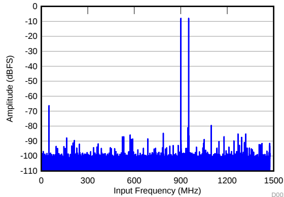
图 15. FFT for Two-Tone Input Signal (–8 dBFS)
