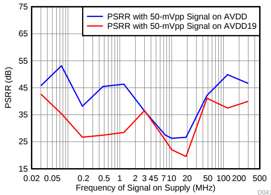
图 65. Power-Supply Rejection Ratio vs Tone Frequency
