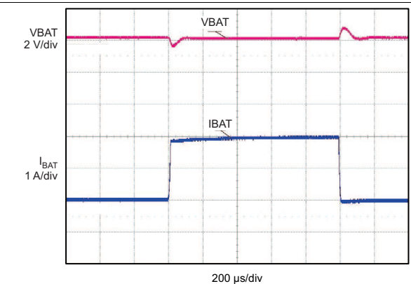
Figure 35. Step Load from 0 to 2 A During Factory Mode
