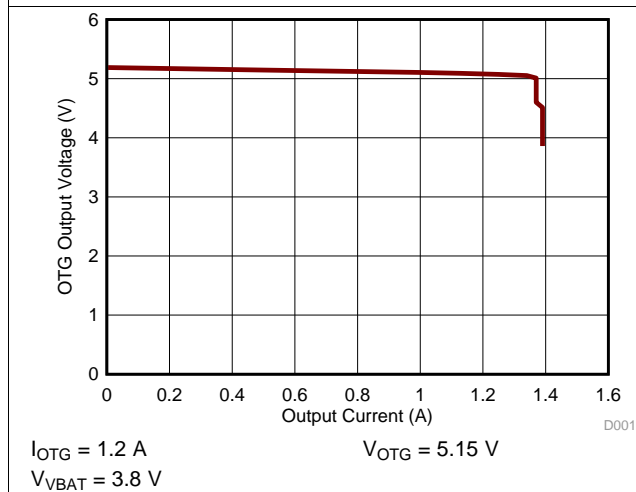
图 3. OTG Output Voltage vs. Output Current
