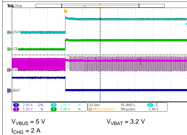
图 38. Charge Disable
