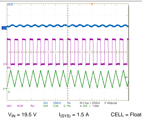
Figure 29. PWM Switching
