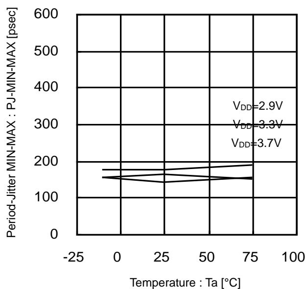
Figure 18. Period-Jitter MIN-MAX vs Temperature (36MHz)
