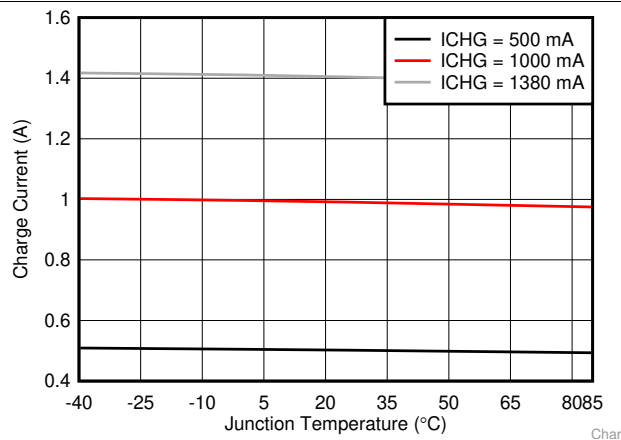
图 5. Charge Current Accuracy
