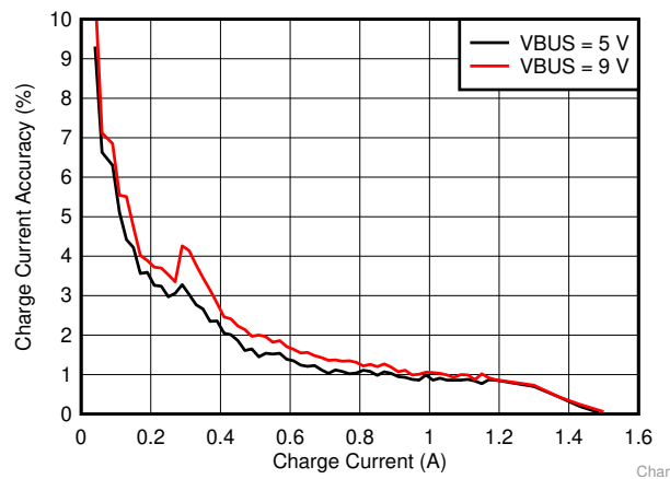
图 5. Charge Current Accuracy
