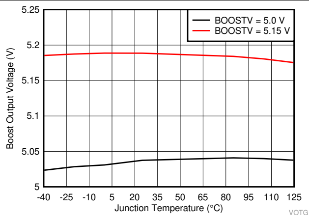
图 11. Boost Output Voltage vs Junction Temperature
