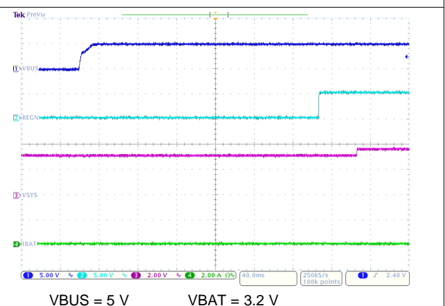
图 43. Power Up with Charge Disabled
