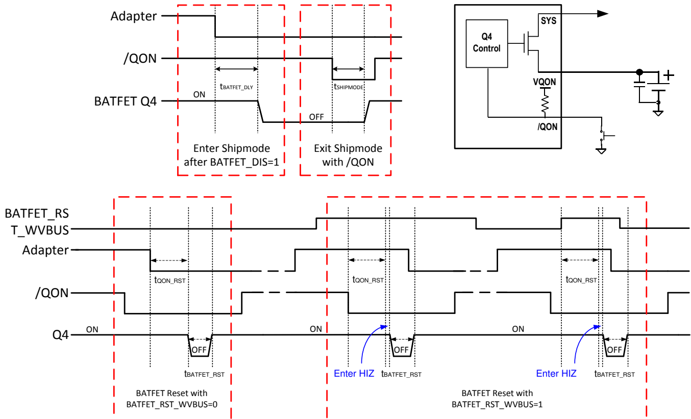
图 16. \overline{\text{QON}} Timing
