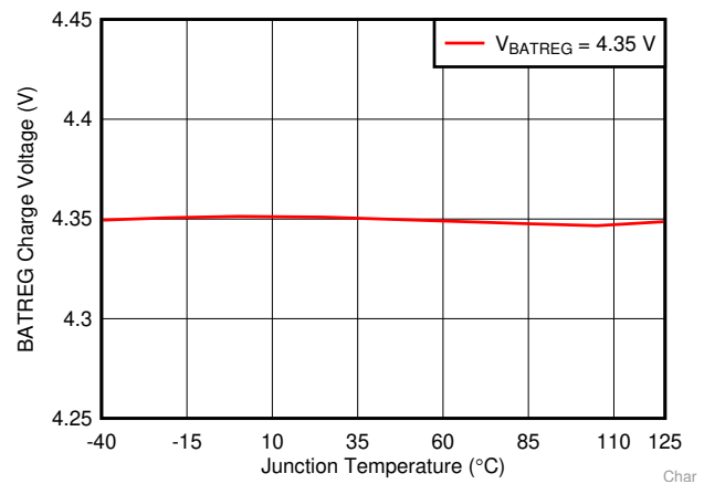
图 6. Battery Charge Voltage vs Junction Temperature
