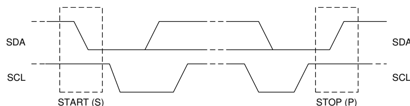
图 18. TS START and STOP conditions
