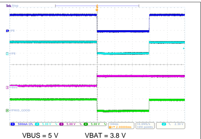
图 41. VBUS Plugged In with Boost Mode Enabled
