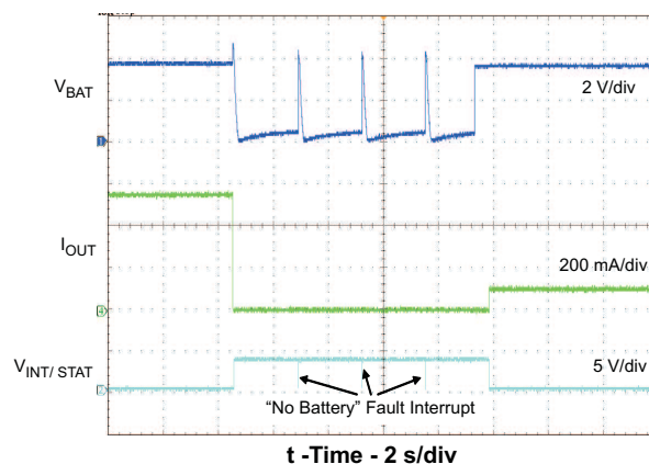
Figure 4. Battery Insertion/Removal
