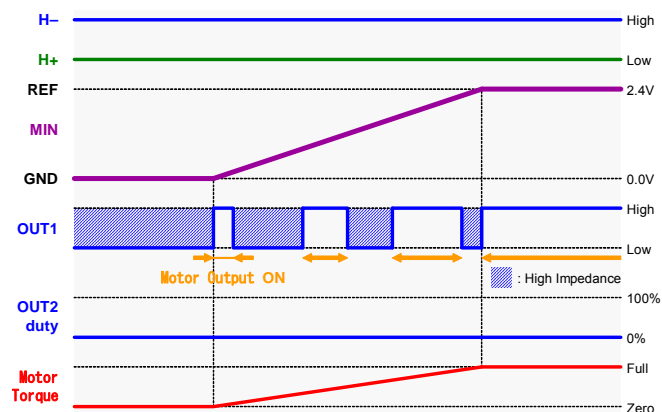
Figure 27. DC Input Operation Timing Chart
