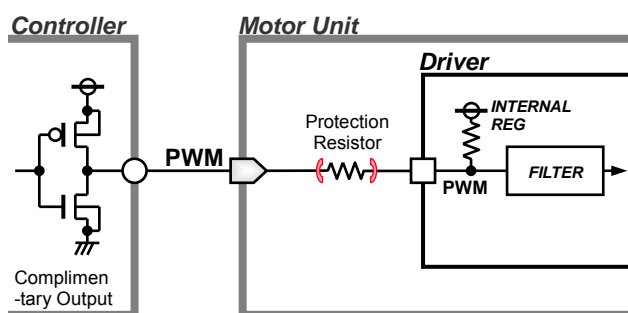
Figure 22. PWM Input Application
