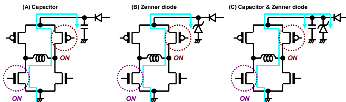
Figure 48. Measure against V_{CC} and Motor Driving Outputs Voltage
