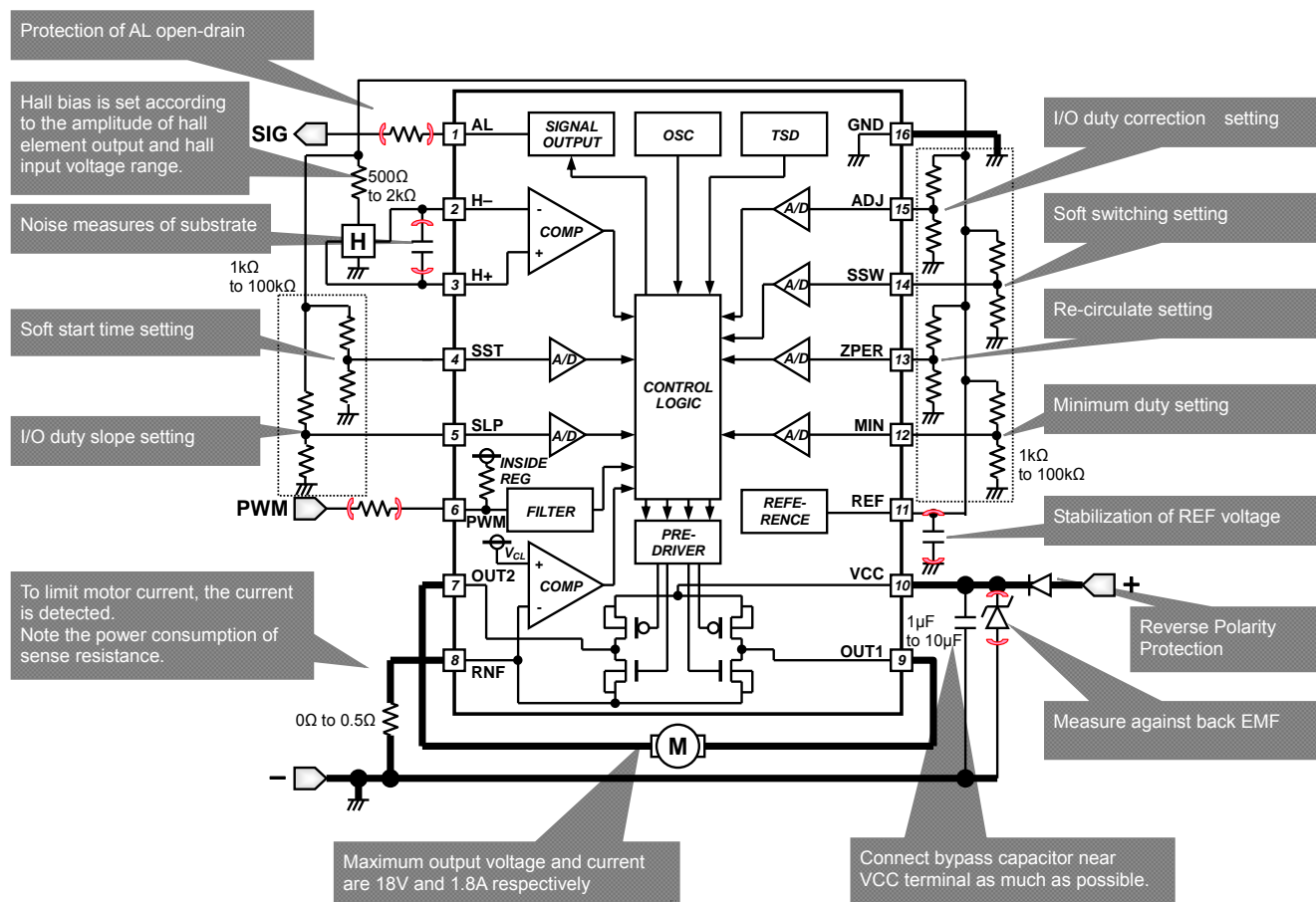
Figure 20. PWM Input Application
