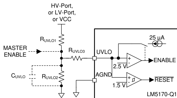
Figure 47. UVLO With Additional Hysteresis Programming
