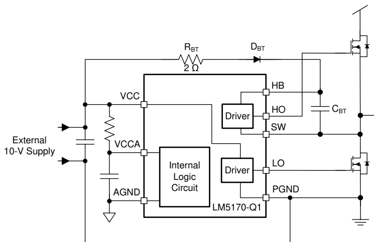
Figure 26. Bootstrap Circuit for High-Side Bias Supply
