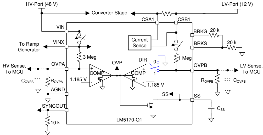
Figure 36. Overvoltage Protection: When Circuit Breaker Function is Not Used
