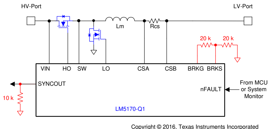
Figure 35. Circuit Breaker Function Disabled
