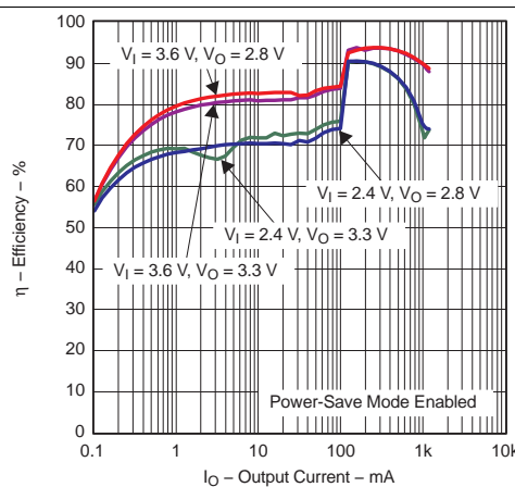
Figure 6. Efficiency vs Output Current (TPS63011)
