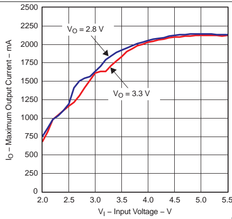
Figure 2. Maximum Output Current vs Input Voltage (TPS63011)
