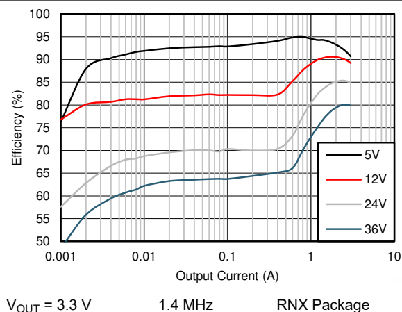
图 8-8. Efficiency
