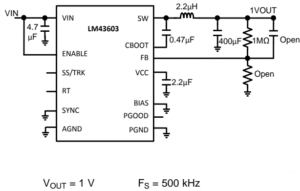
Figure 49. BOM for V_{OUT} = 1\text{ V} F_S = 500\text{ kHz}
