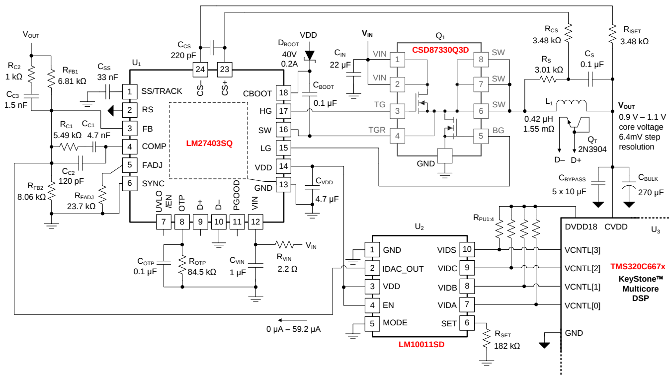
图 48. Application Circuit 3 with V_{IN} = 3\text{ V to }20\text{ V} , V_{OUT} = 0.9\text{ V to }1.1\text{ V} , I_{OUT(max)} = 15\text{ A} , F_{SW} = 450\text{ kHz}
