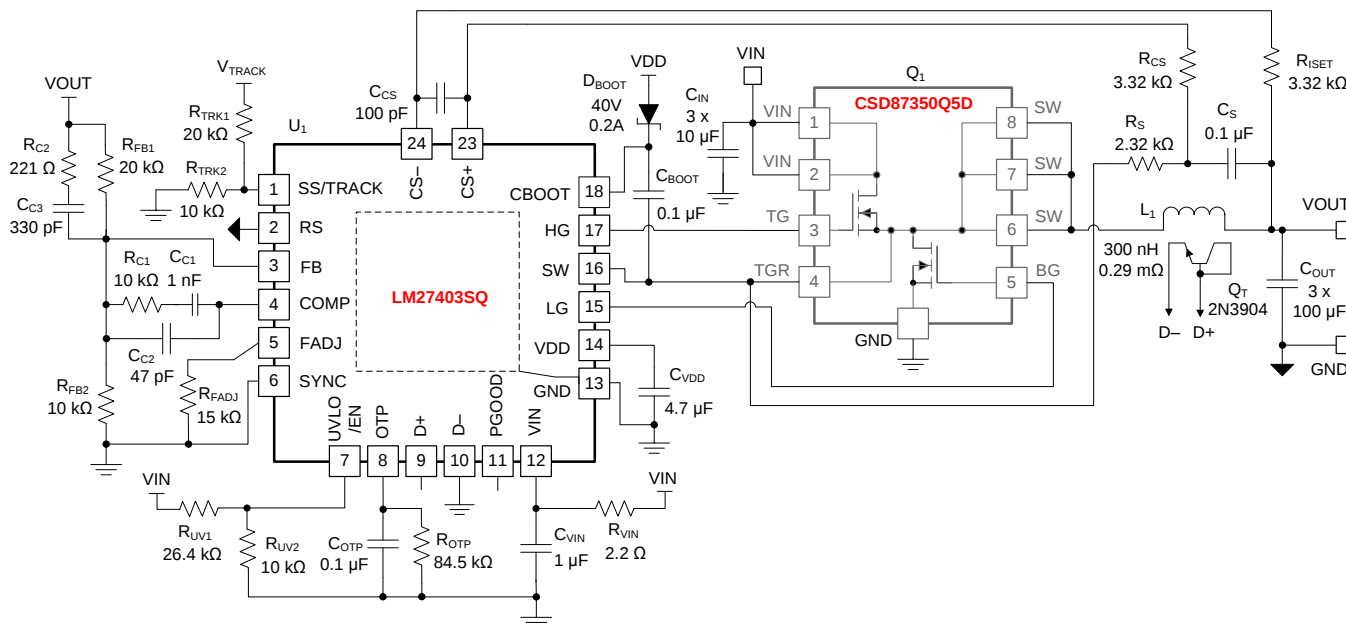
图 46. Application Circuit 2 With V_{IN} = 4.5\text{ V} to 15\text{ V} ( V_{IN(nom)} = 12\text{ V} ), V_{OUT} = 1.8\text{ V} , I_{OUT(max)} = 30\text{ A} , F_{SW} = 600\text{ kHz}
