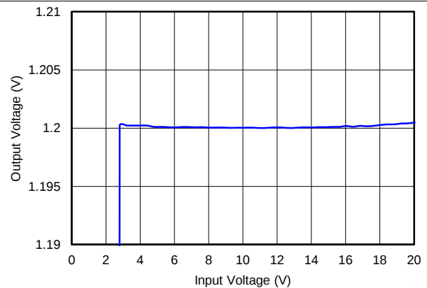
图 4. Line Regulation
