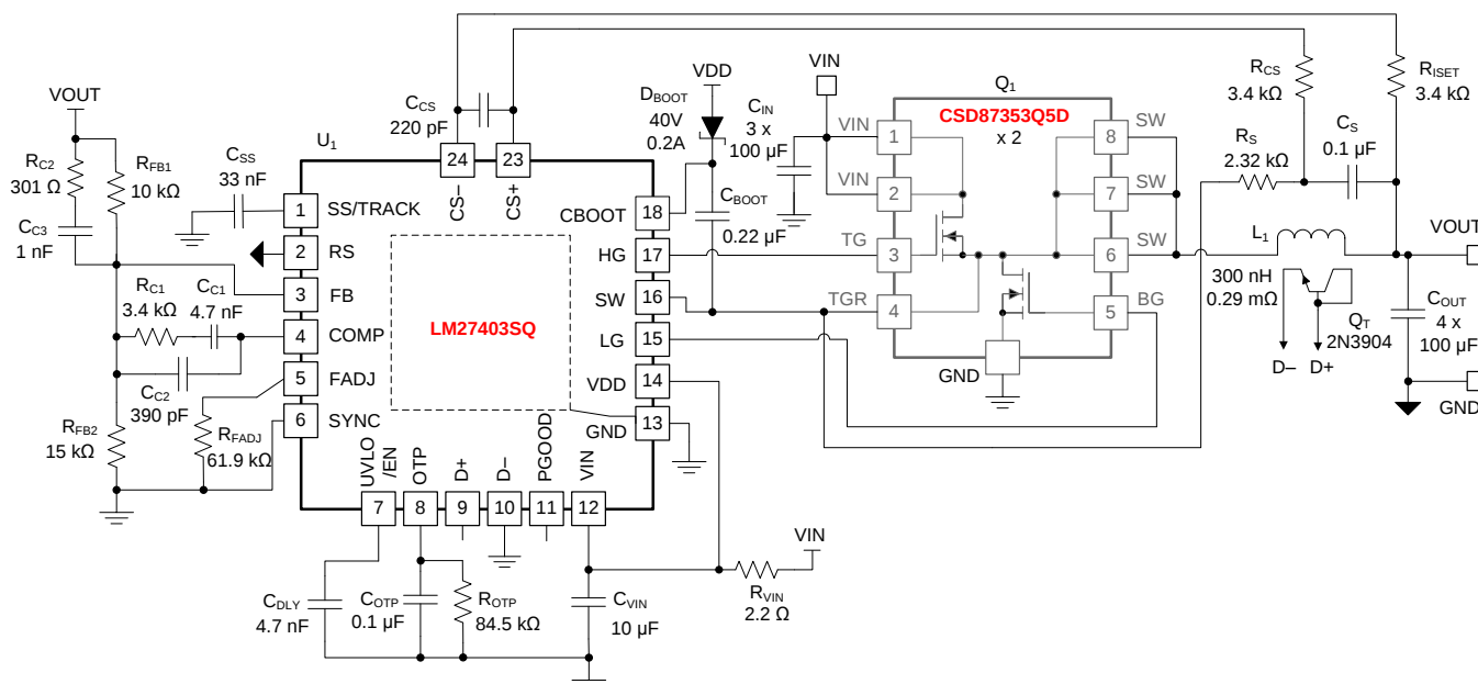
图 50. Application Circuit 5 With V_{IN} = 3.3\text{ V} to 5.5\text{ V} , V_{OUT} = 1\text{ V} , I_{OUT(max)} = 25\text{ A} , F_{SW} = 250\text{ kHz}
