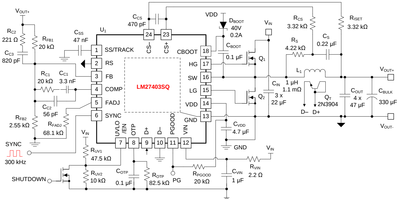
图 41. Application Circuit 1 with V_{IN} = 6.5\text{ V to }20\text{ V} ( V_{IN(nom)} = 12\text{ V} ), V_{OUT} = 0.6\text{ V to }5.3\text{ V} , I_{OUT(max)} = 25\text{ A} , F_{SW} = 300\text{ kHz} (Using External Synchronization Signal)
