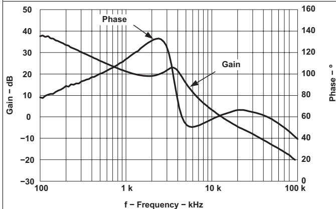
图 18. Overall Gain and Phase vs. Frequency
