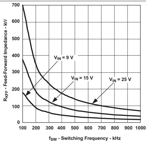
图 2. Feed-Forward Impedance vs. Switching Frequency
