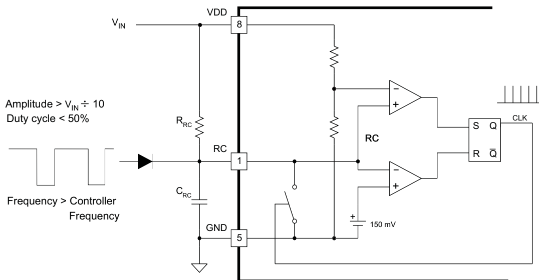
Figure 25. Diode-Connected Synchronization
