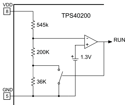
Figure 29. Undervoltage Lockout
