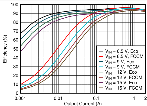
Figure 8-2. Efficiency
