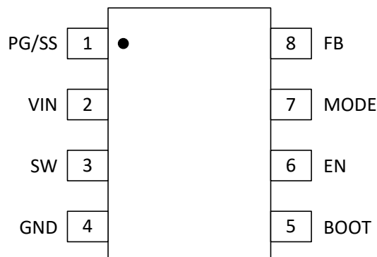
8-Pin SOT583 DRL Package (Top View)
