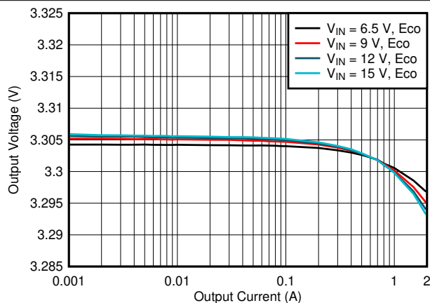
Figure 8-3. Load Regulation
