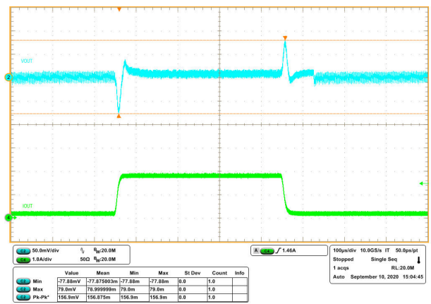
Figure 8-13. Transient Response 0.2 to 1.8 A with Slew Rate of 0.25 A/ \mu s (Eco-mode)
