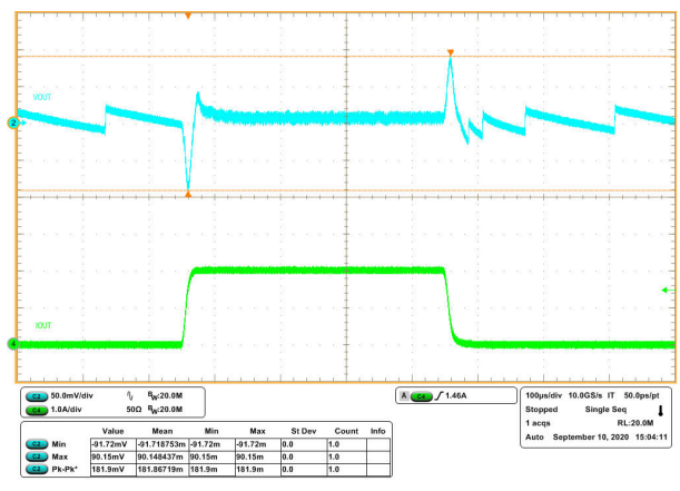
Figure 8-11. Transient Response 0 to 2 A with Slew Rate of 0.25 A/ \mu s (Eco-mode)
