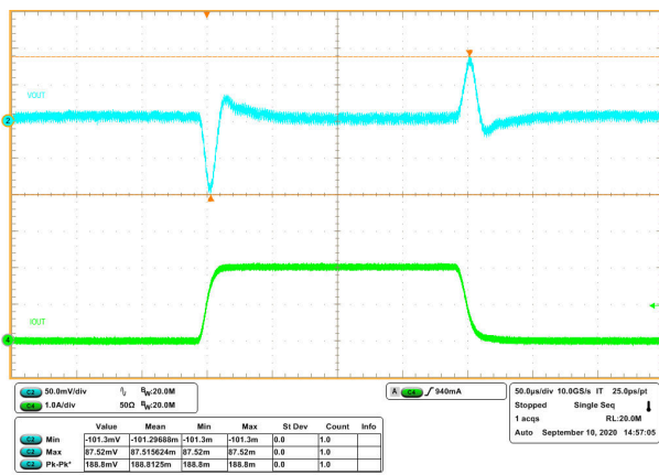
Figure 8-12. Transient Response 0 to 2 A with Slew Rate of 0.25A/ \mu s (FCCM)
