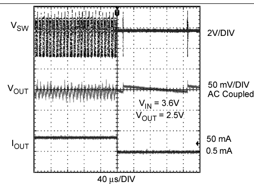
Figure 22. Load Transient Response
