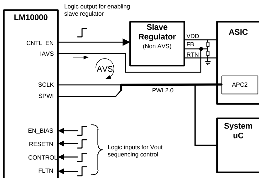
Figure 7. LM10000 provides flexible digital power management via multi-master PWI 2.0, and flexible V_{OUT} sequencing control
