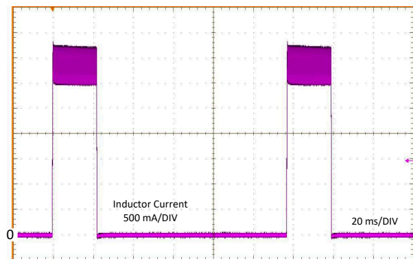
图 8-13. Inductor Current Burst in Short-Circuit Mode; LM63625
