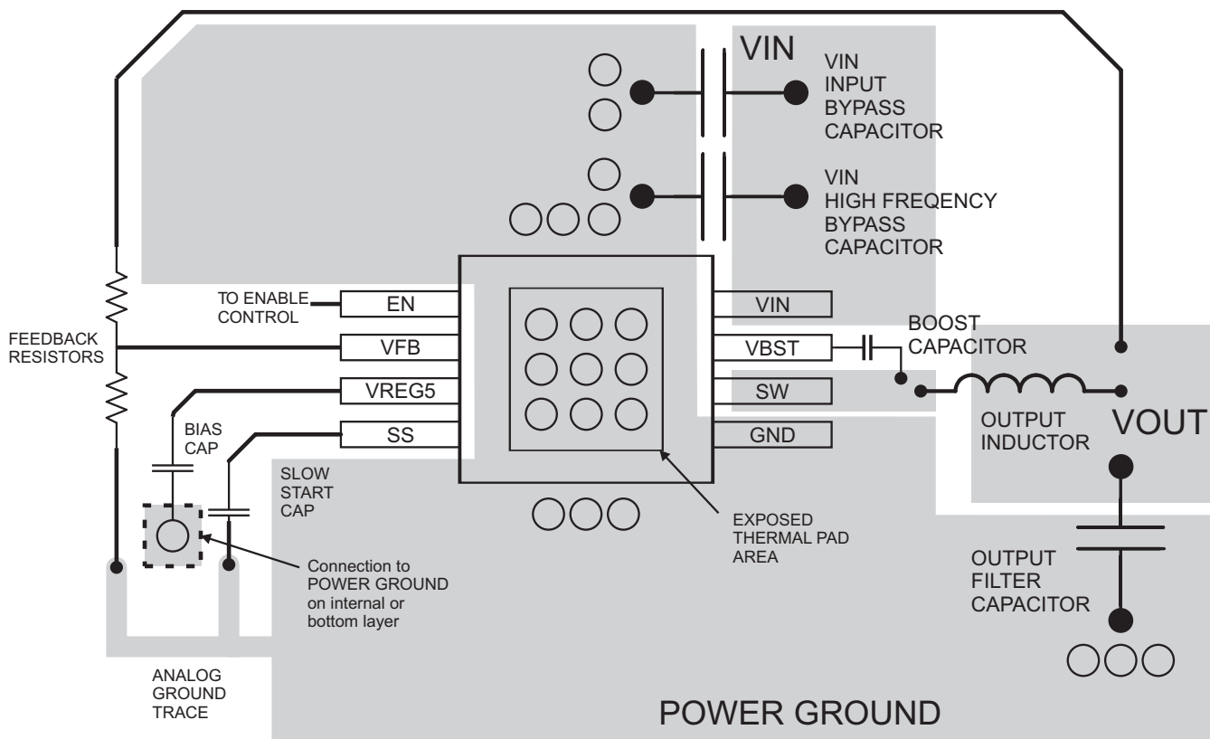
Figure 18. PCB Layout
