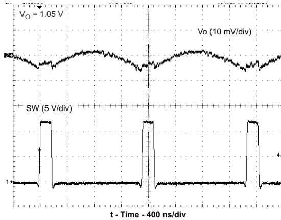
Figure 13. VOLTAGE RIPPLE AT OUTPUT ( I_O = 2 A)
