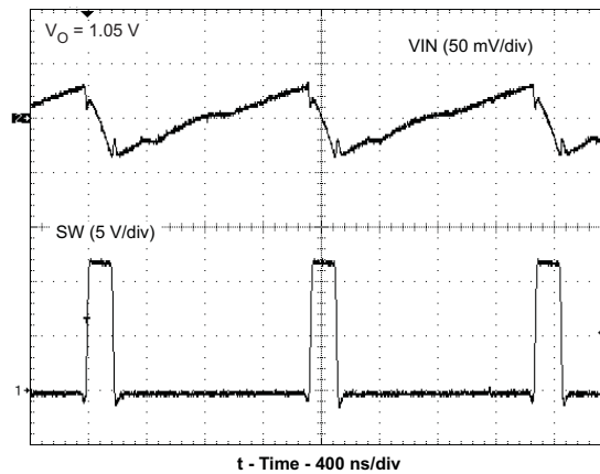
Figure 15. VOLTAGE RIPPLE AT INPUT ( I_O = 2 A)
