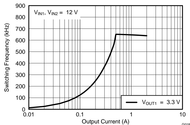
Figure 18. V_{O1} = 3.3\text{V} , SW-frequency vs Output Current (PWP)
