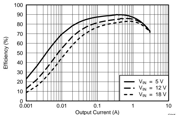
Figure 15. V_{O2} = 1.5\text{V} , Efficiency vs Output Current
