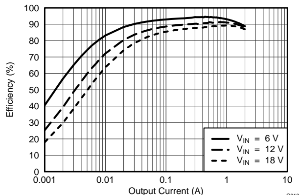
Figure 13. V_{O1} = 1.5\text{V} , Efficiency vs Output Current
