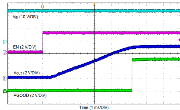
Figure 9-2. Start-up by EN
