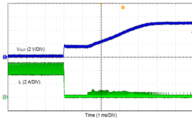
Figure 9-9. Output Short Recovery
