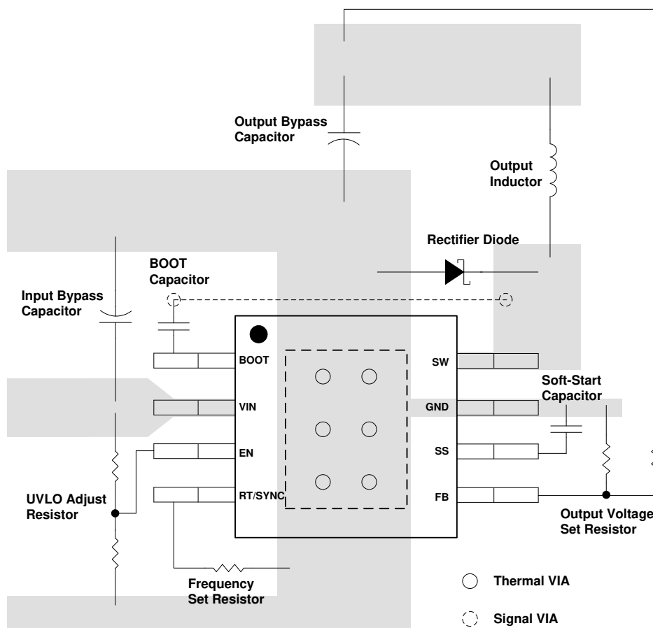
Figure 11-1. Layout
