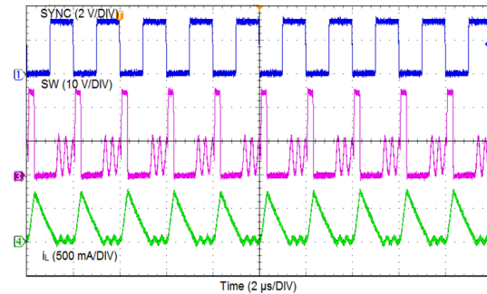
Figure 8-7. Synchronizing in DCM
