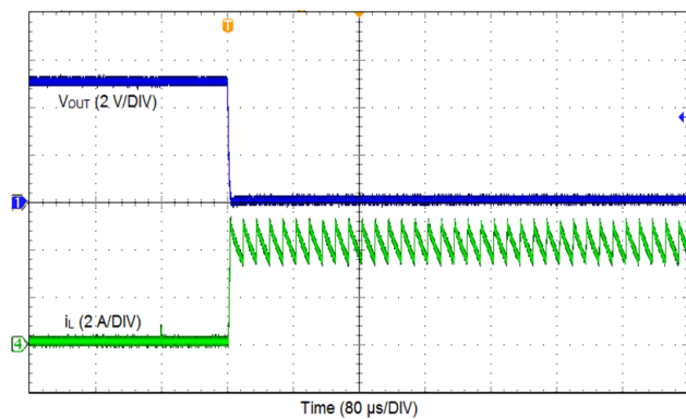
Figure 9-8. Output Short
