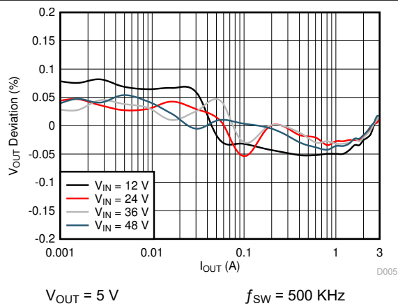
Figure 7-5. Load Regulation
