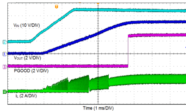
Figure 9-3. Start-up By V_{IN}
