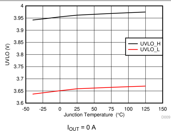
Figure 7-10. UVLO Threshold
