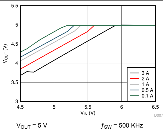
Figure 7-7. Dropout Curve
