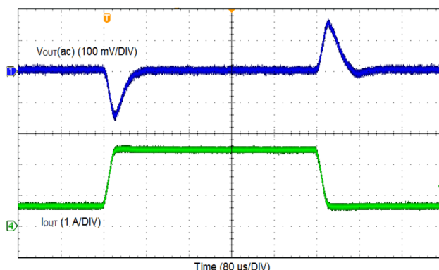
Figure 9-5. DCM Mode
