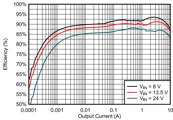
图 9-12. Efficiency
