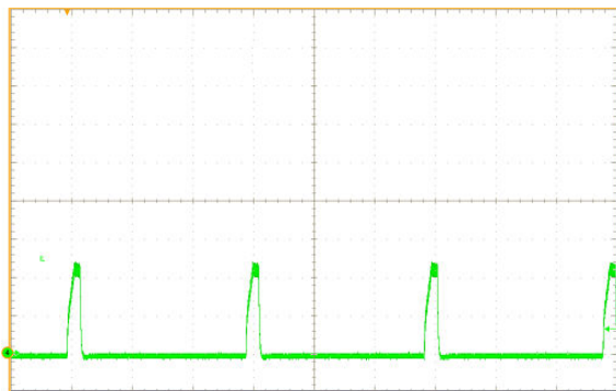
图 8-16. Inductor Current Bursts During Hiccup
