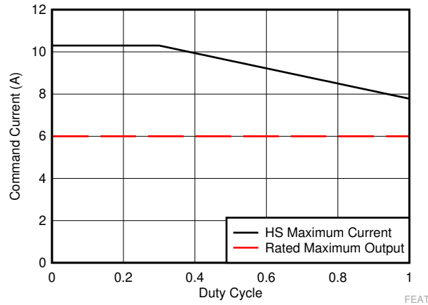
图 8-13. Maximum Current Allowed Through the HS FET - Function of Duty Factor for LM62460-Q1
