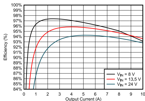
EVM 效率 ( \Theta_{JA} = 21.6^{\circ}\text{C/W} ) : V_{OUT} = 5\text{V} , F_{SW} = 0.4\text{MHz}
