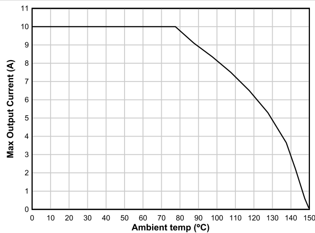
图 9-4. Maximum Output Current versus Ambient Temperature
