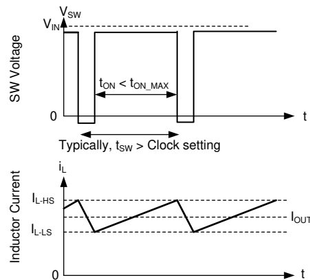
图 8-14. Current Limit Waveforms
