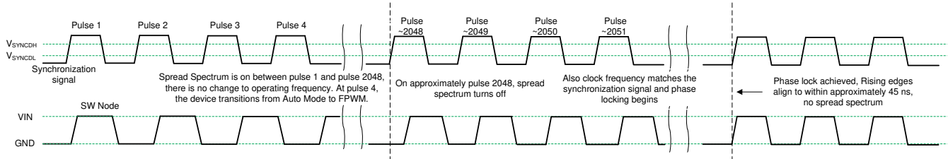
图 8-5. Synchronization Process
