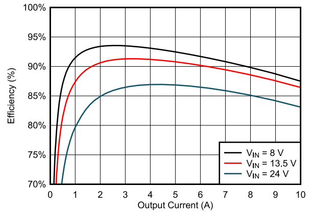
图 9-13. Efficiency
