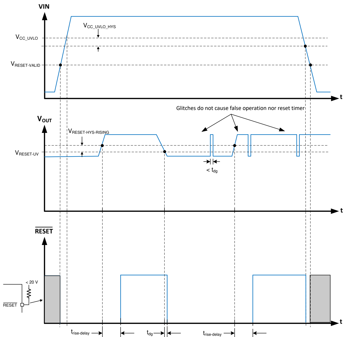
图 8-8. \overline{RESET} Timing Diagram (Excludes OV Events)
