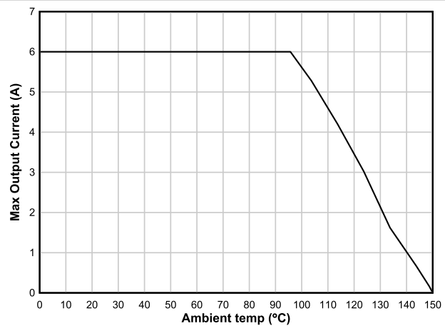
图 9-5. Maximum Output Current versus Ambient Temperature
