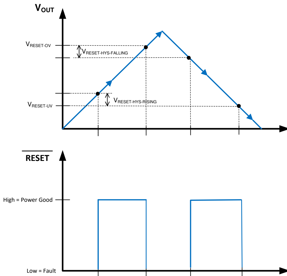
图 8-7. \overline{\text{RESET}} Static Voltage Thresholds
