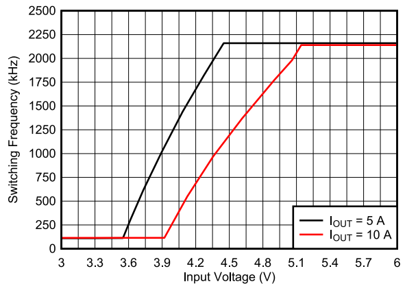
图 9-27. Frequency Dropout
