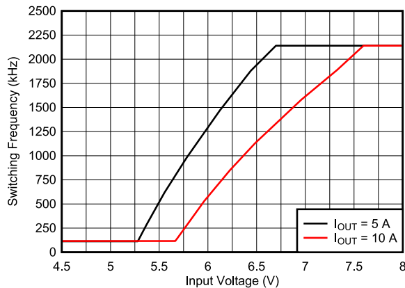
图 9-26. Frequency Dropout
