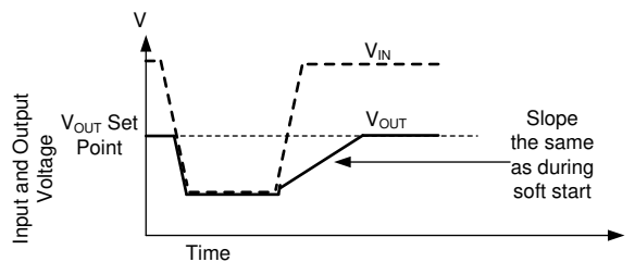
图 8-25. When Output Voltage Falls, It Recovers Slowly Preventing Overshoot and Large Inrush Currents
