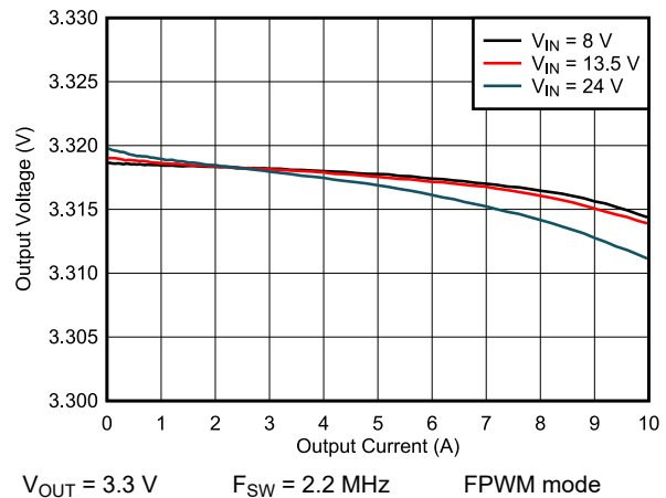
图 9-21. Load and Line Regulation
