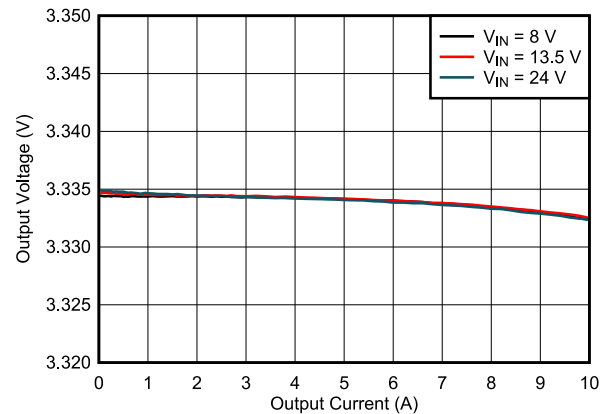
图 9-15. Load and Line Regulation
