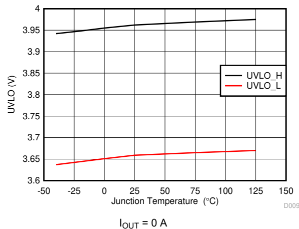
Figure 6-12. UVLO Threshold
