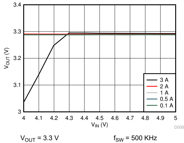
Figure 6-7. Dropout Curve
