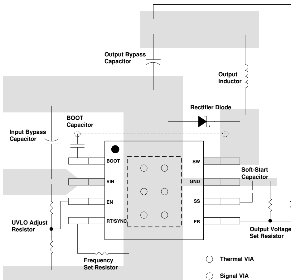
Figure 10-1. Layout
