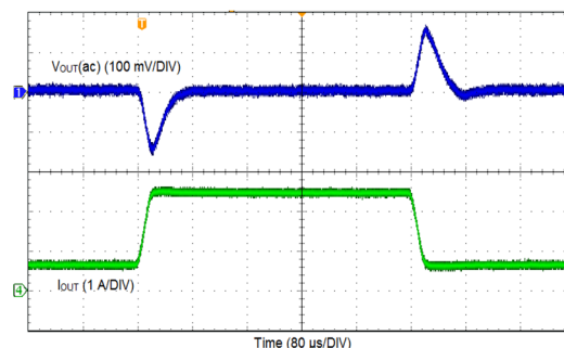
Figure 8-5. DCM Mode
