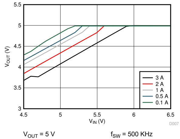
Figure 6-8. Dropout Curve
