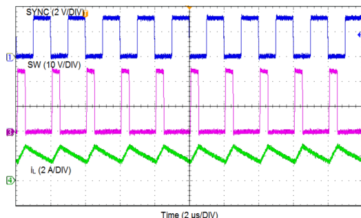
Figure 7-6. Synchronizing in CCM
