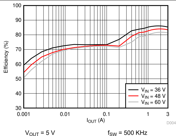
Figure 6-4. Efficiency vs. Load Current
