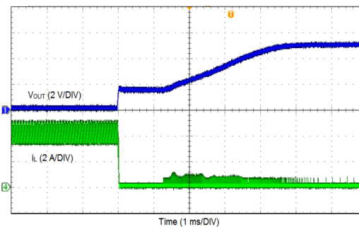
Figure 8-9. Output Short Recovery
