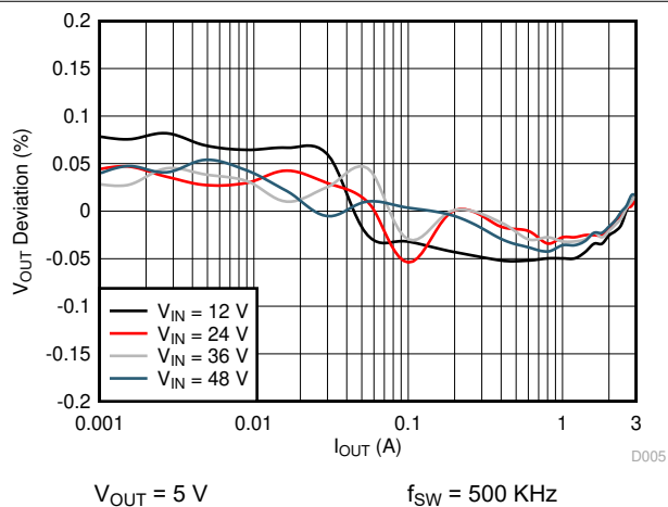
Figure 6-5. Load Regulation
