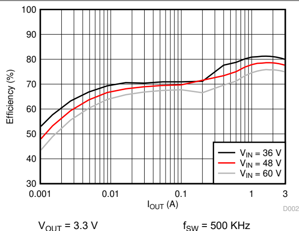
Figure 6-2. Efficiency vs. Load Current
