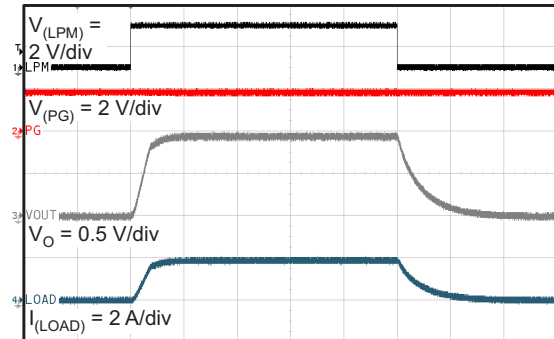
V_{(LPM)} = 2\text{ V}/\text{div} V_{(PG)} = 2\text{ V}/\text{div} V_O = 0.5\text{ V}/\text{div} I_{(LOAD)} = 2\text{ A}/\text{div} Time = 50 \mu\text{s}/\text{div} R_{(LOAD)} = 0.47\ \Omega
