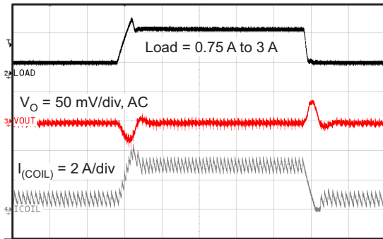
V_O = 0.95\text{ V} Time = 10 \mu\text{s}/\text{div}
