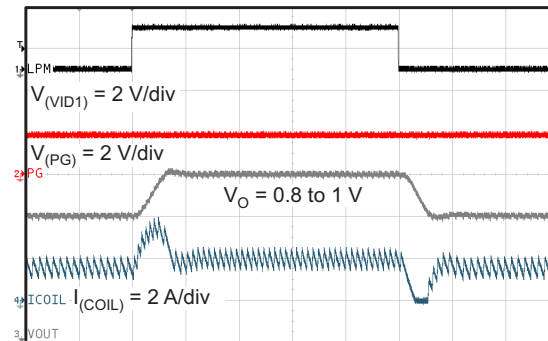
Time = 10 \mu\text{s}/\text{div} R_{(LOAD)} = 0.47\ \Omega
