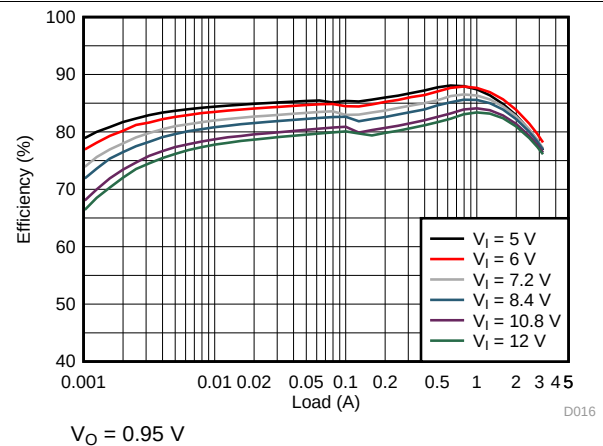
图 6. TPS62134B Efficiency
