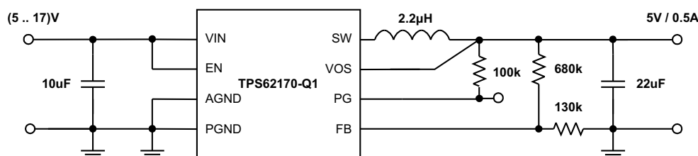
Figure 31. 5-V/0.5-A Power Supply
