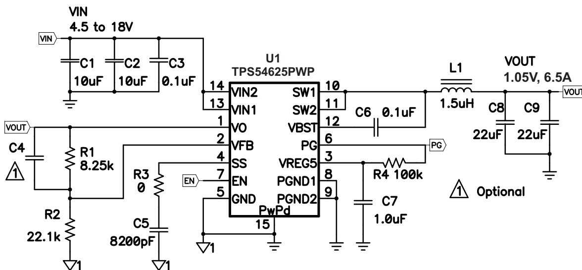
Figure 15. Schematic
