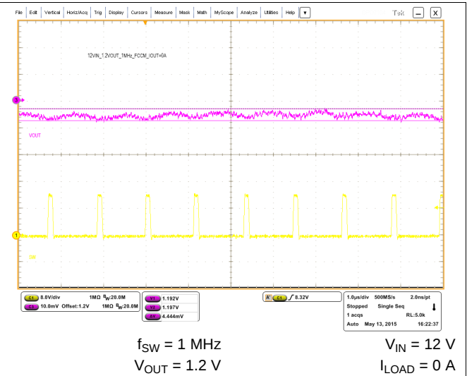
图 13. FFCM Steady-State Operation
