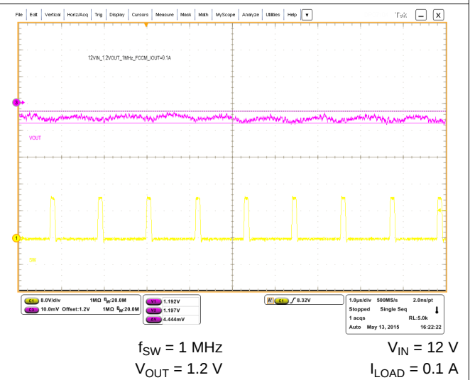
图 15. Steady-State Operation
