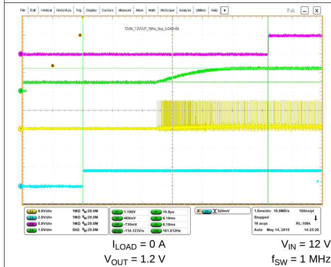
图 22. Skip Mode Pre-Bias Start-Up
