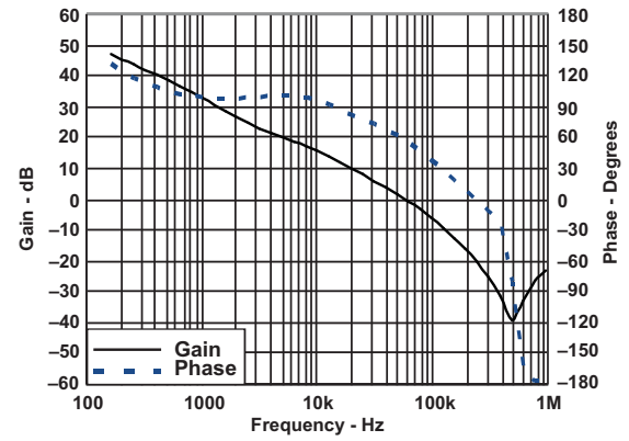
Figure 47. Closed-Loop Response
