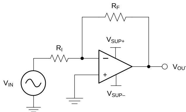
图 21. Application Schematic
