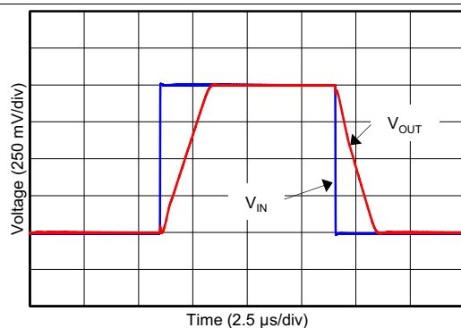
图 14. Small-Signal Pulse Response (Maximum Supply)
