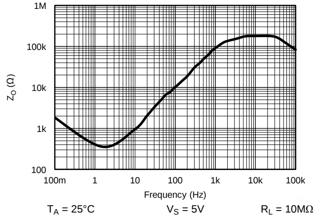
Figure 32. 开环输出阻抗
