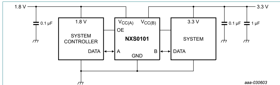
Fig. 9. Typical operating circuit
