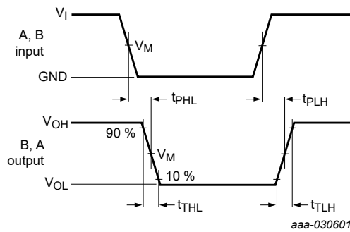
Fig. 5. The data input (An, Bn) to data output (Bn, An) propagation delay times
