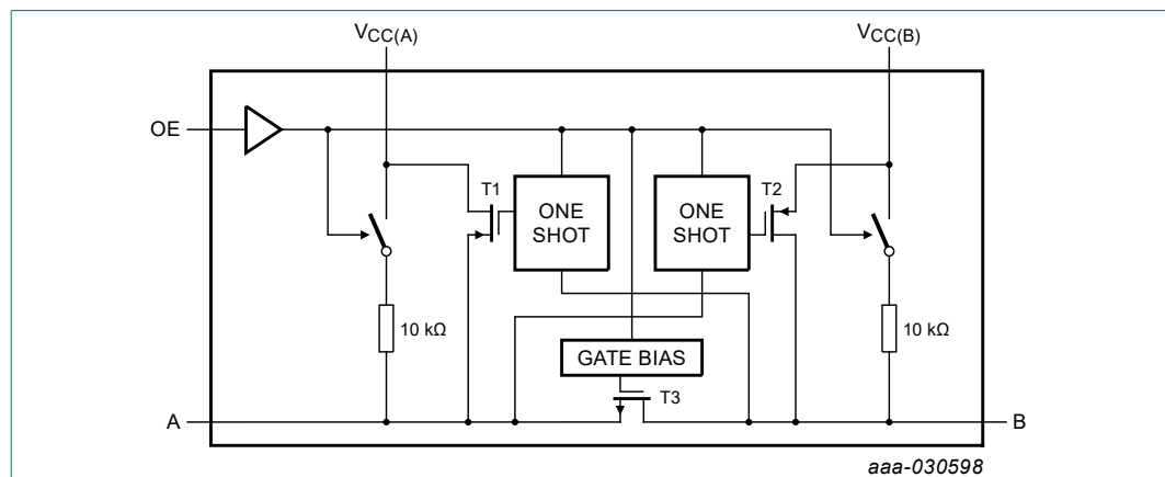
Fig. 10. Architecture of NXS0101 I/O cell
