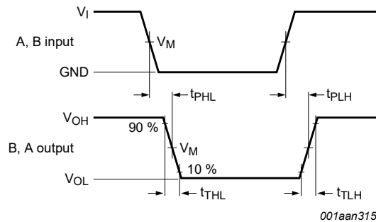
Fig. 4. The data input (An, Bn) to data output (Bn, An) propagation delay times
