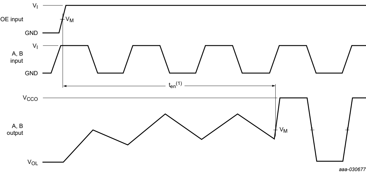
Fig. 5. Disable times
