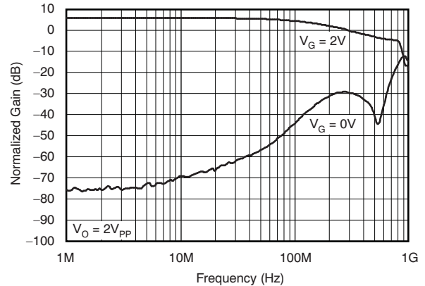
Figure 24. Frequency Response
