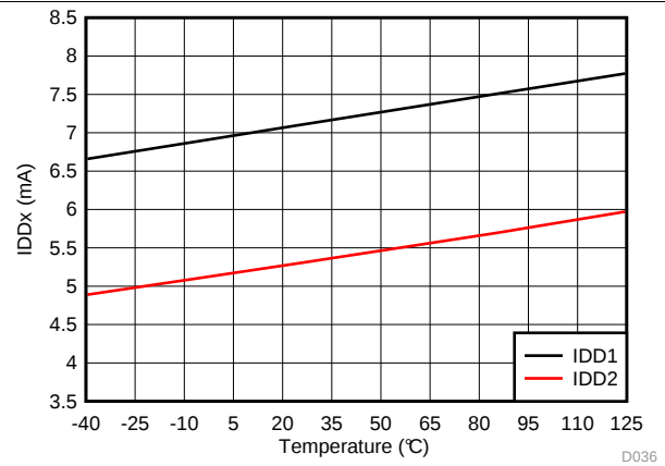
图 36. Supply Current vs Temperature
