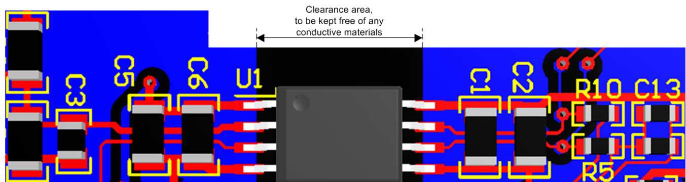
图 49. Recommended Layout of the AMC1211A-Q1
