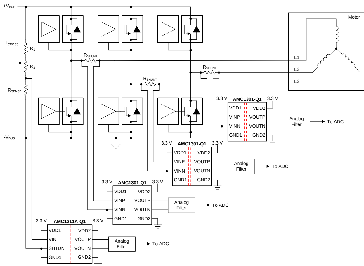
图 45. Using the AMC1211A-Q1 for DC Bus Voltage Sensing in Traction Inverters
