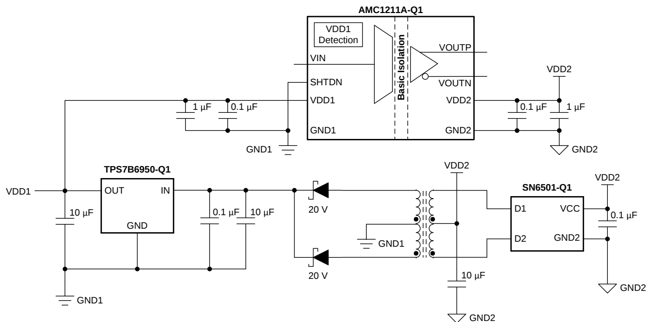
图 48. SN6501-Q1-Based, High-Side Power Supply
