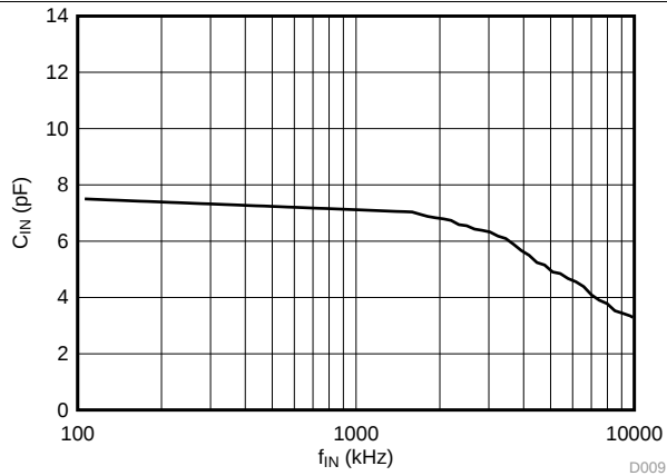
图 11. Input Capacitance vs Input Signal Frequency
