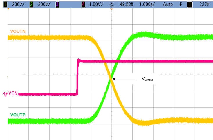
图 47. Step Response of the AMC1211A-Q1
