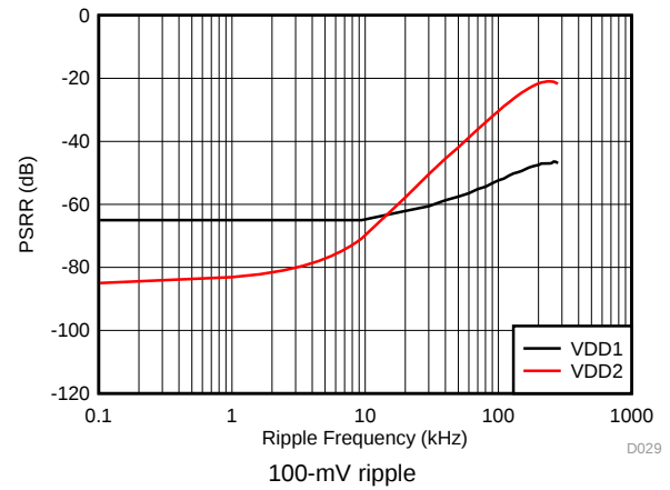
图 30. Power-Supply Rejection Ratio vs Ripple Frequency
