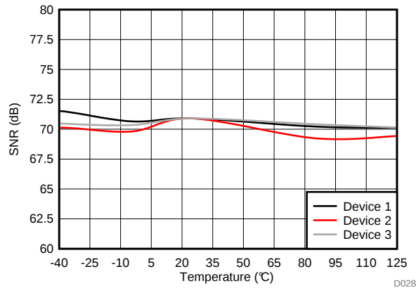
图 29. Signal-to-Noise Ratio vs Temperature
