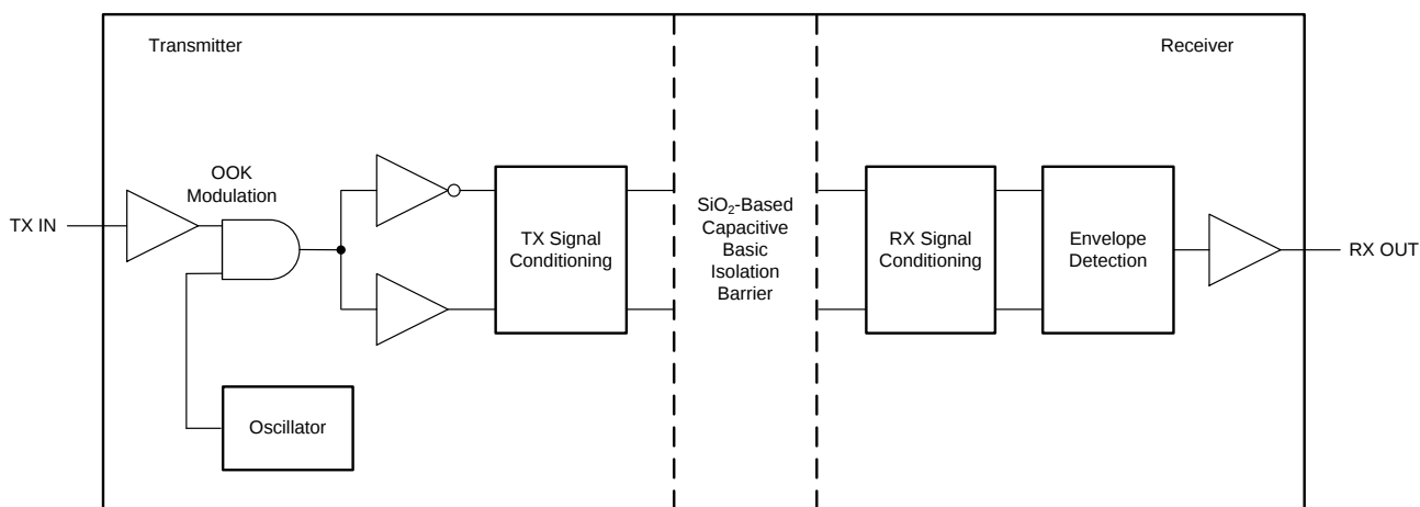
图 42. Block Diagram of an Isolation Channel
