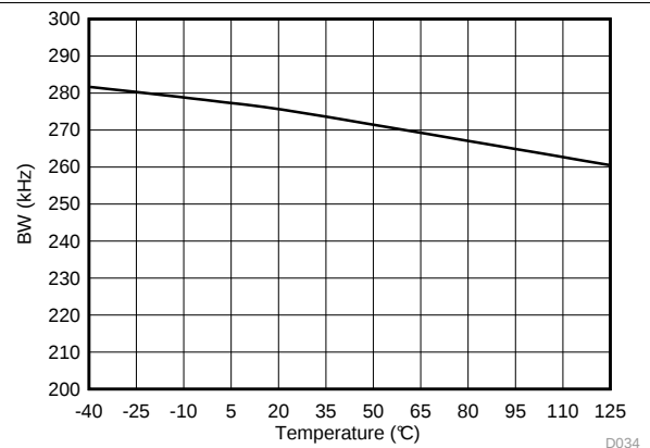
图 34. Output Bandwidth vs Temperature
