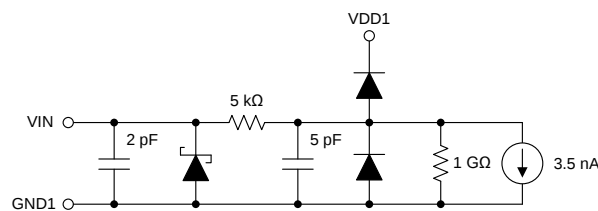
图 41. Equivalent Analog Input Circuit
