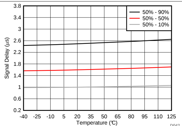
图 40. VIN to VOUTP, VOUTN Signal Delay vs Temperature
