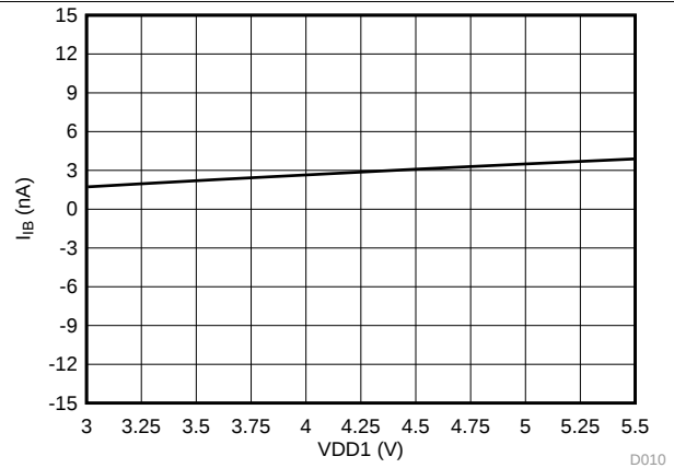
图 12. Input Bias Current vs High-Side Supply Voltage
