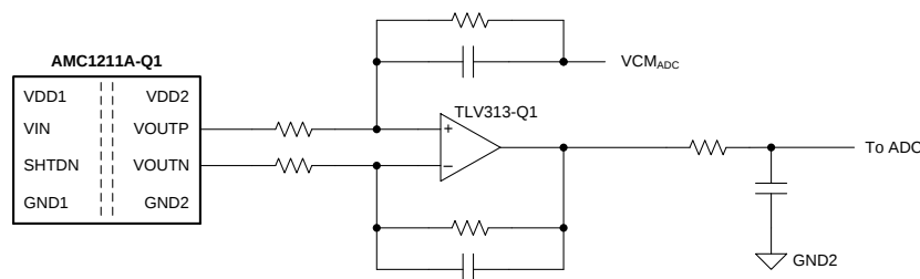
图 46. Connecting the AMC1211A-Q1 Output to Single-Ended Input ADC
