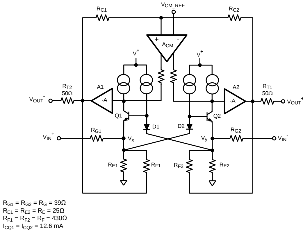
Figure 24. Block Diagram
