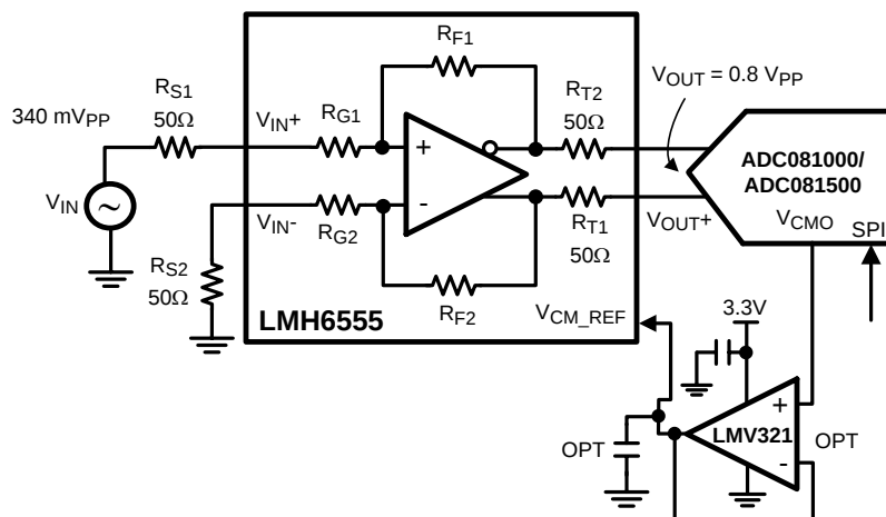
Figure 23. Single Ended to Differential Conversion
