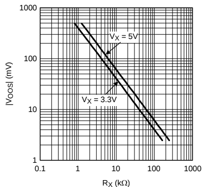
Figure 32. LMH6555 Differential Output Shift Due to R_X in Figure 31
