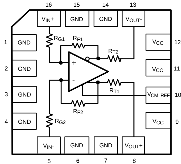
Figure 2. 16-Pin WQFN
