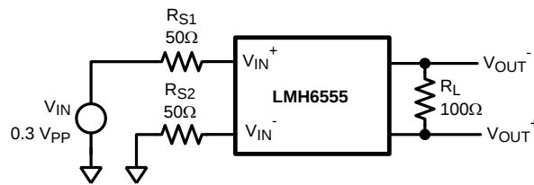
Figure 46. Single Ended Input Drive
