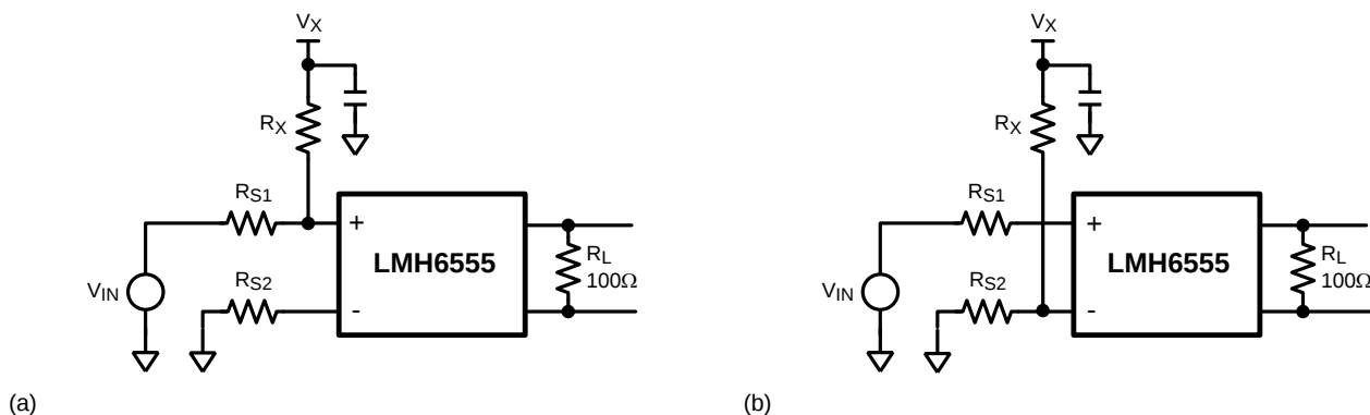
Figure 31. Differential Output Shift Circuits
