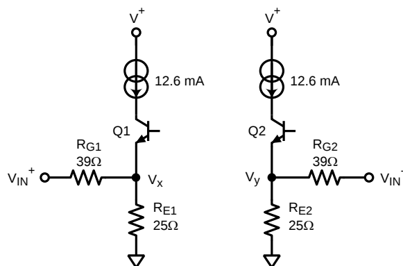
Figure 45. Equivalent Input Stage
