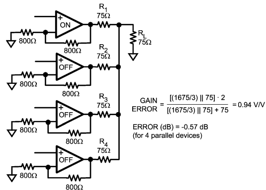
Figure 22. Multiplexer Input Expansion by Combining Outputs
