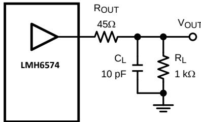
Figure 28. Decoupling Capacitive Loads
