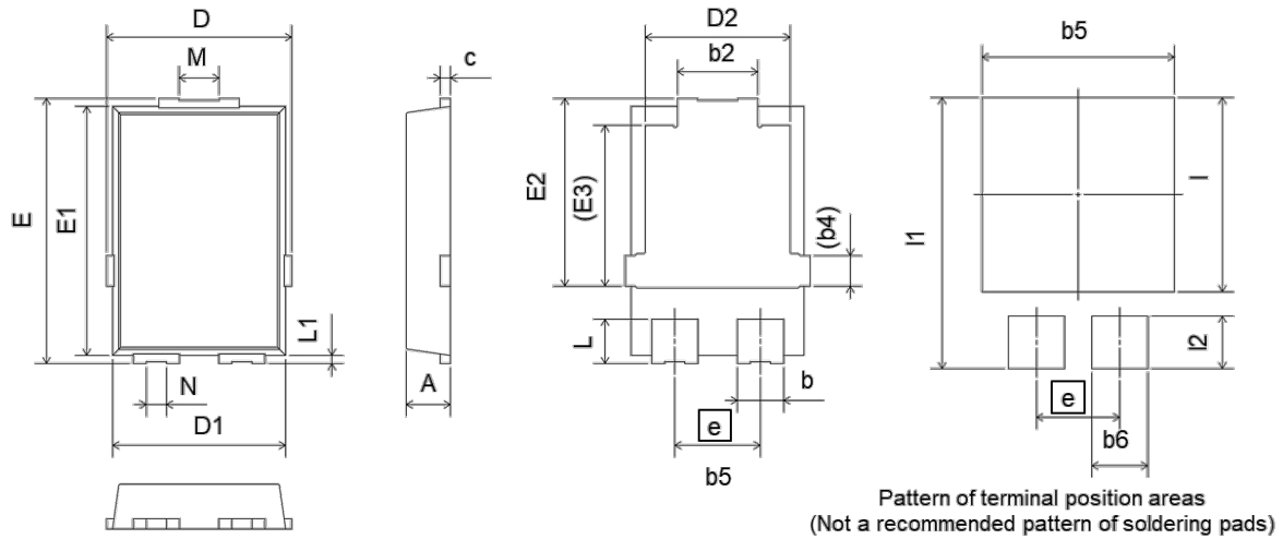
TO-277A, (TO-277GE)
