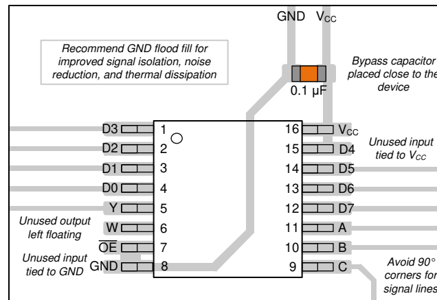
Figure 11-1. Example layout for the SN74HCS251 in the PW package.
