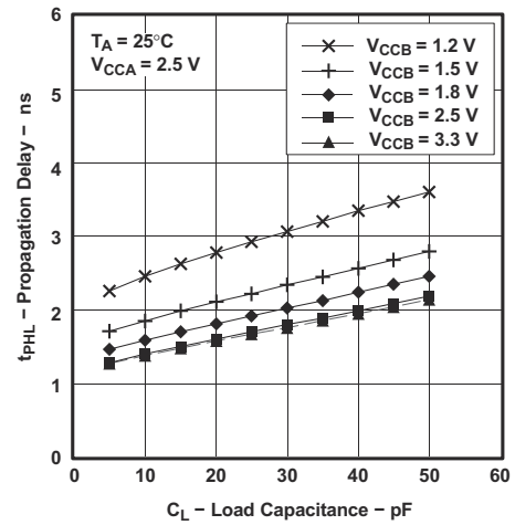
图 7-8. Typical Propagation Delay t_{PLH} (A to B) vs Load Capacitance
