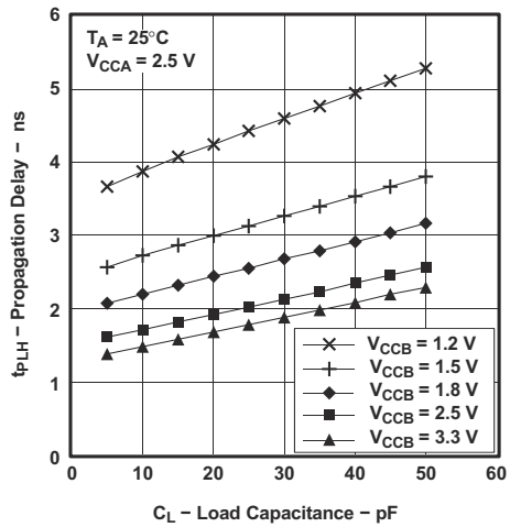
图 7-7. Typical Propagation Delay t_{PLH} (A to B) vs Load Capacitance
