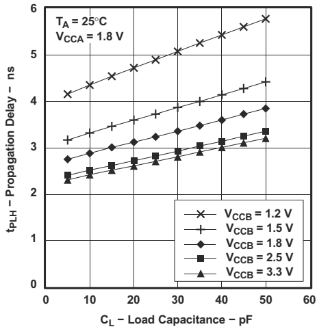
图 7-5. Typical Propagation Delay t_{PLH} (A to B) vs Load Capacitance
