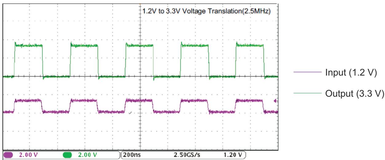
图 10-2. Translation Up (1.2 V to 3.3 V) at 2.5 MHz
