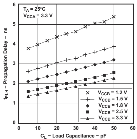
图 7-9. Typical Propagation Delay t_{PLH} (A to B) vs Load Capacitance
