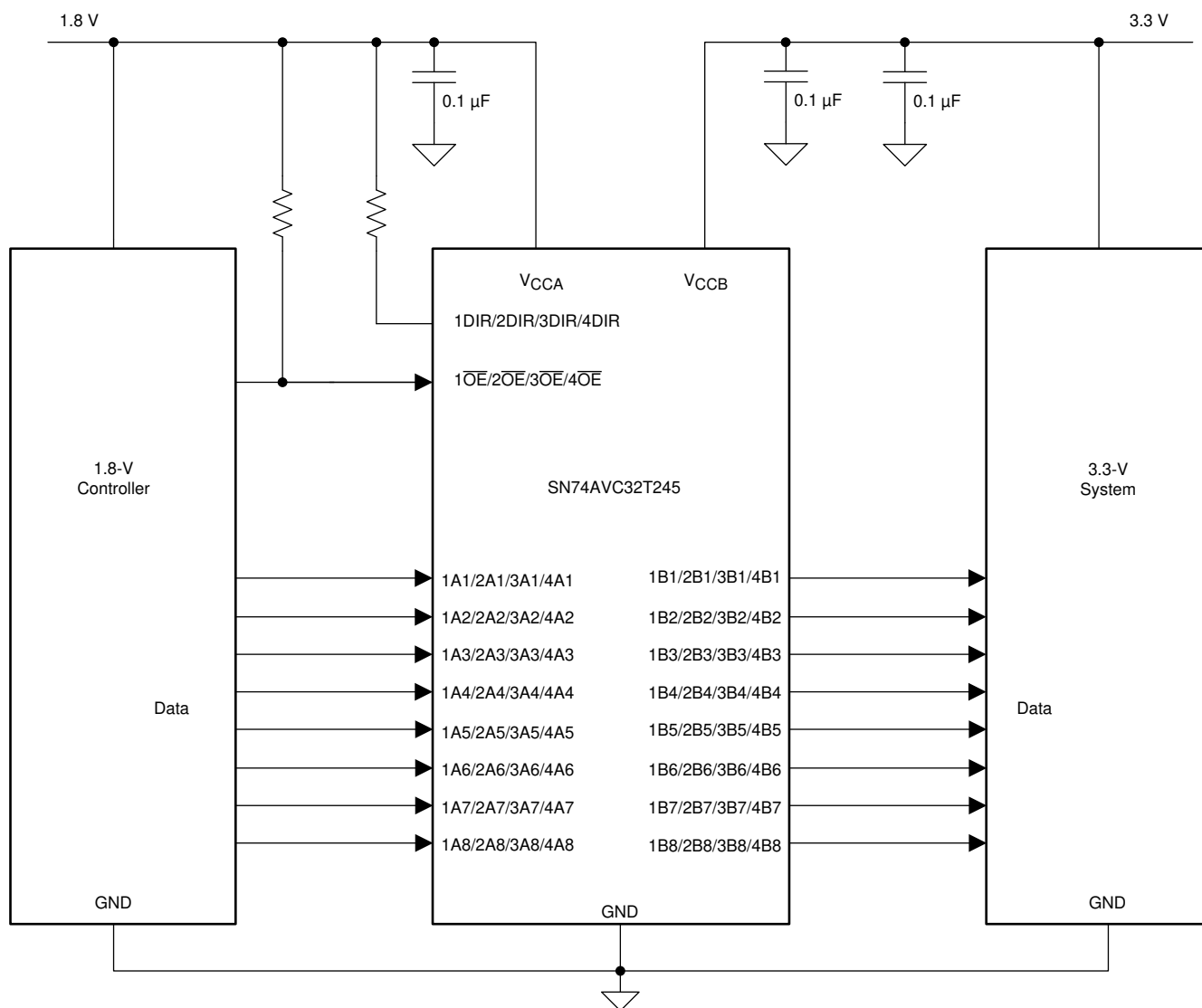
图 10-1. Application Schematic
