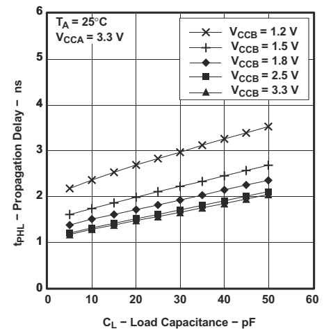
图 7-10. Propagation Delay vs Load Capacitance
