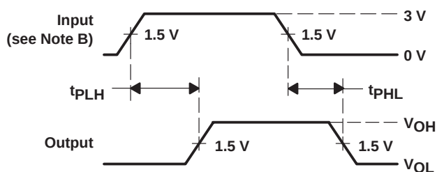
VOLTAGE WAVEFORM 4 PROPAGATION DELAY TIMES (ENn to A port) †
