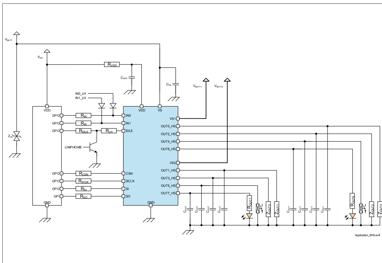
Figure 1 TLE75080-ESD Application Diagram
