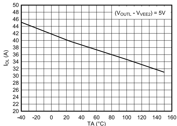
Figure 6-2. I OLTL vs. Temperature
