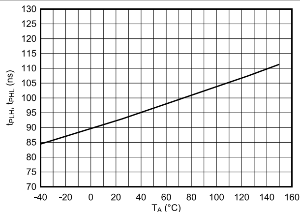
Figure 6-7. Propagation Delay vs. Temperature
