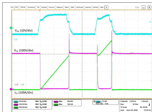
Figure 8-5. IGBT Double Pulse Waveform
