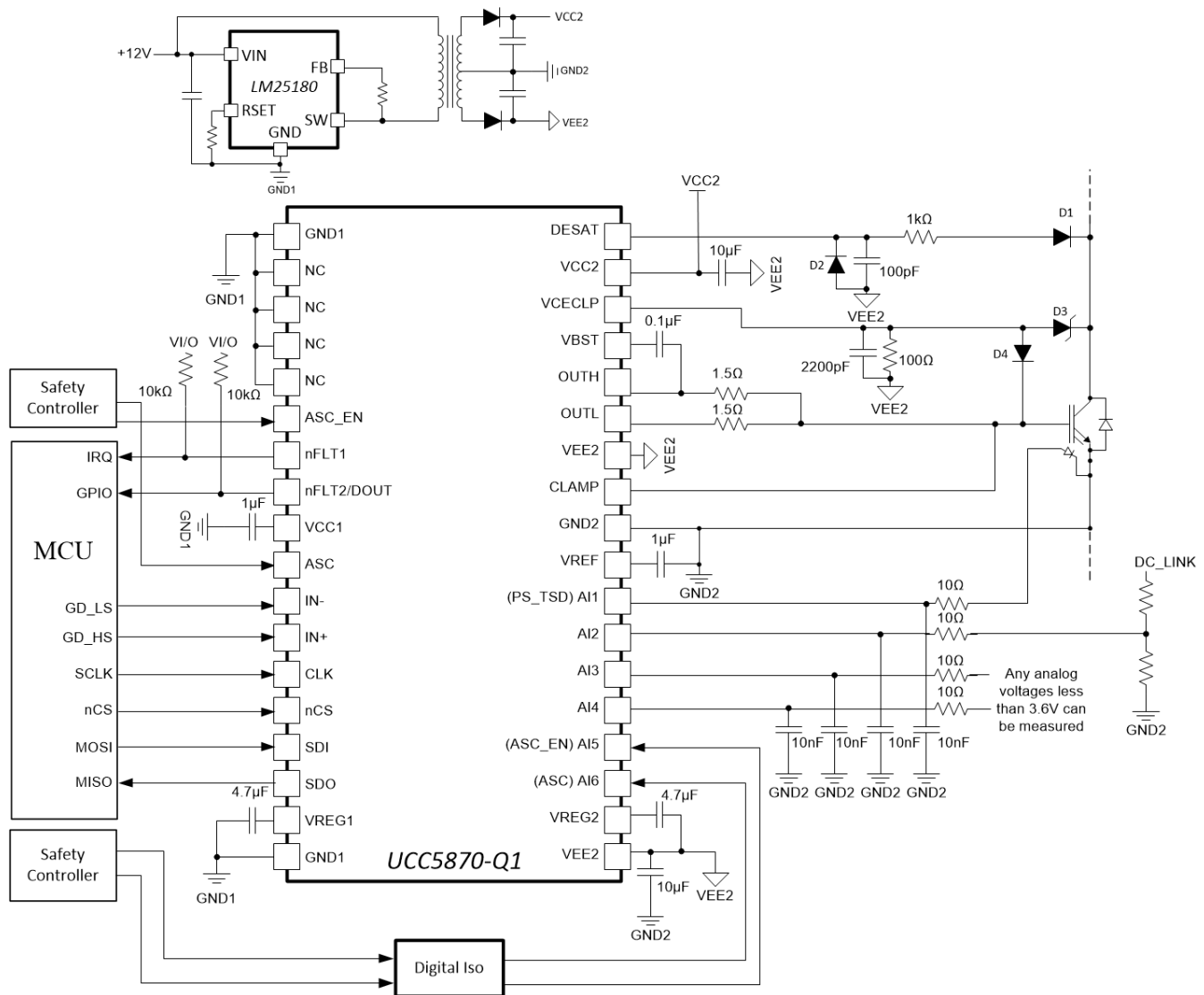
Figure 8-8. Typical Application Circuits of UCC5870-Q1 using DESAT Overcurrent Protection
