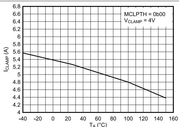
Figure 6-4. Internal Miller Clamp Current vs. Temperature
