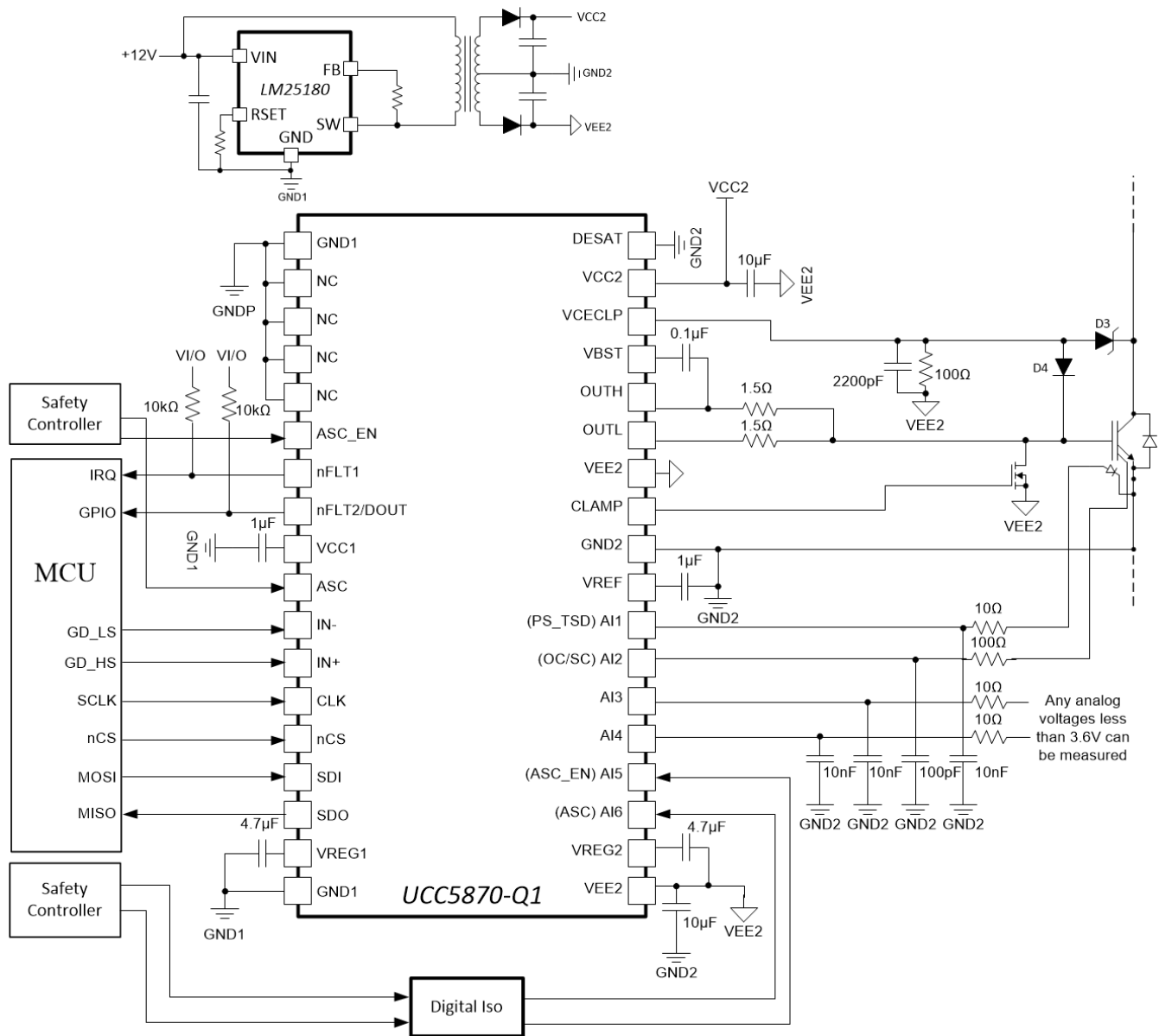
Figure 8-3. Typical Application Circuit of UCC5870-Q1 using Sense FET Overcurrent Sensing
