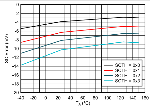
Figure 6-17. SC Threshold Error vs. Temperature
