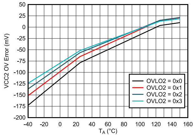
Figure 6-13. VCC2 OVLO Error vs. Temperature
