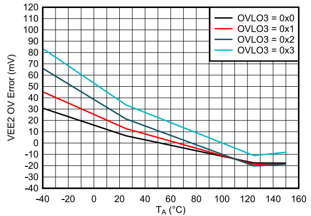
Figure 6-14. VEE2 OVLO Error vs. Temperature
