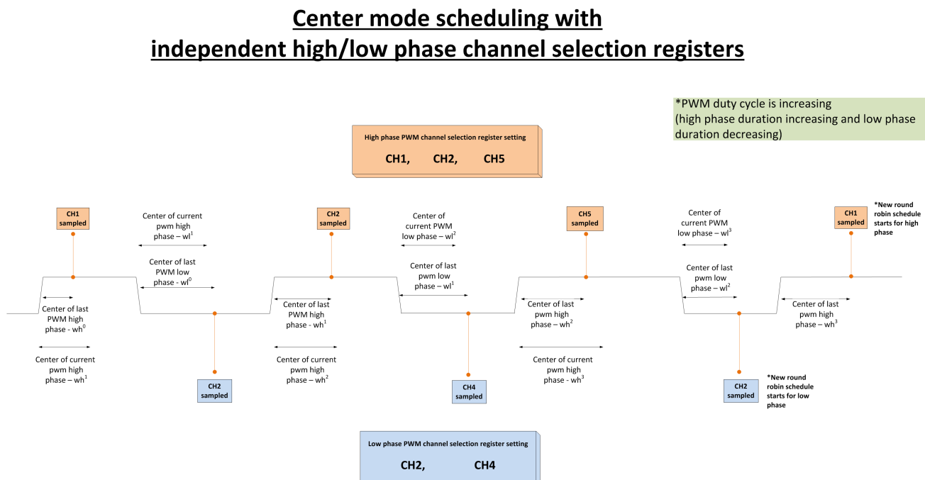
Figure 7-4. ADC center sampling mode
