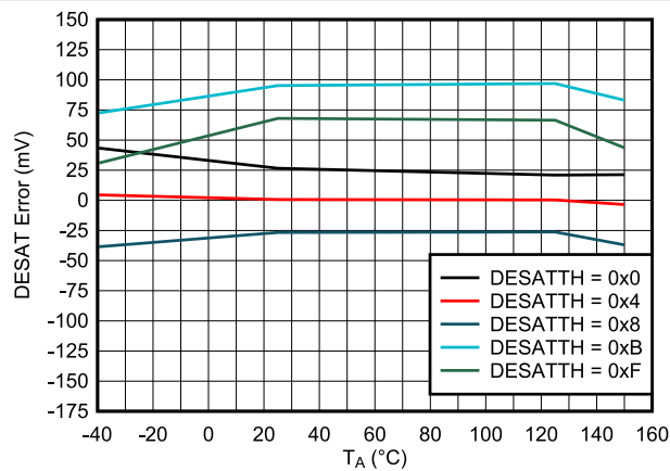
Figure 6-15. DESAT Threshold Error vs. Temperature
