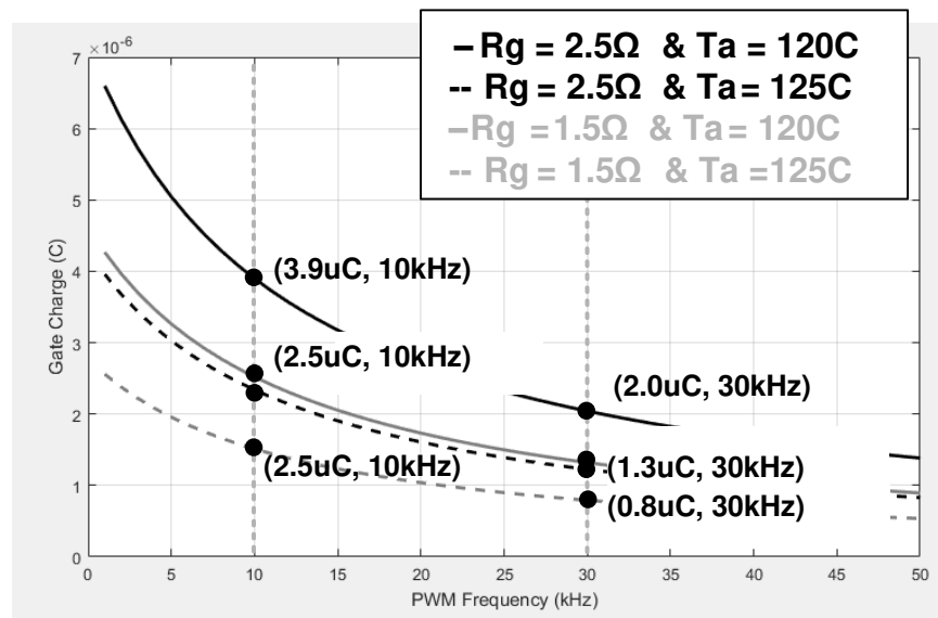
Figure 8-1. Relationship of power transistor gate charge vs PWM frequency under different conditions of R_g and T_A .
