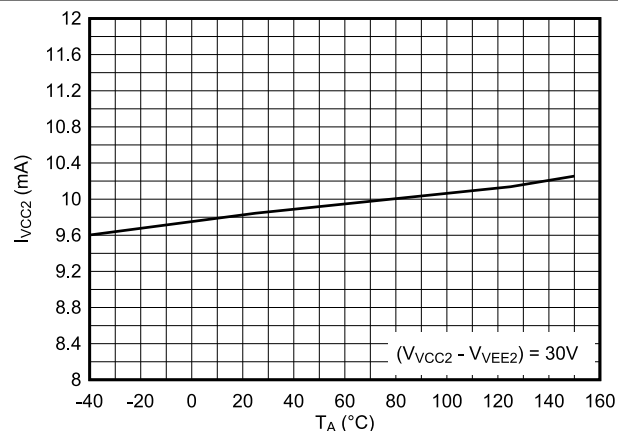
Figure 6-6. VCC2 Quiescent Current vs. Temperature
