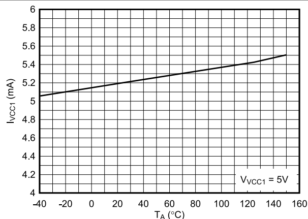
Figure 6-5. VCC1 Quiescent Current vs. Temperature
