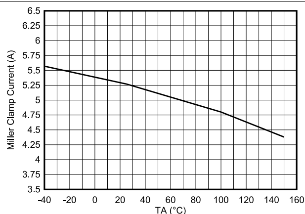
Figure 6-3. Internal Miller Clamp Sink Current vs. Temperature
