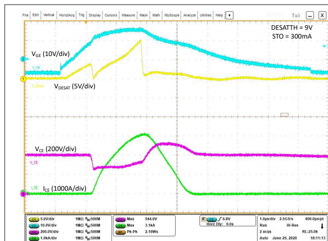
Figure 8-10. Soft Turn-Off (STO) Shutdown Response to DESAT Event
