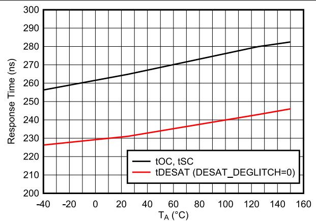
Figure 6-18. Overcurrent Protection Response Time vs. Temperature
