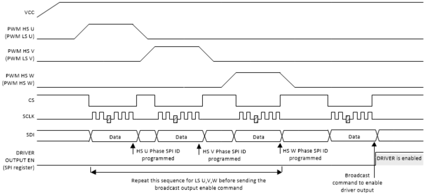
Figure 8-2. Timing diagram for addressing when using the Address-based SPI Communication Scheme.
