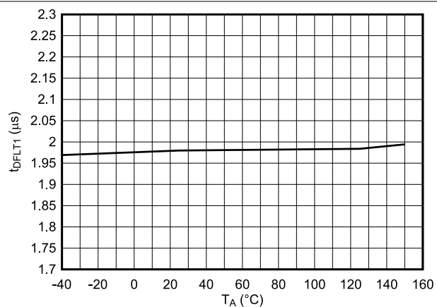
Figure 6-20. nFLT1 Response Time vs Temperature
