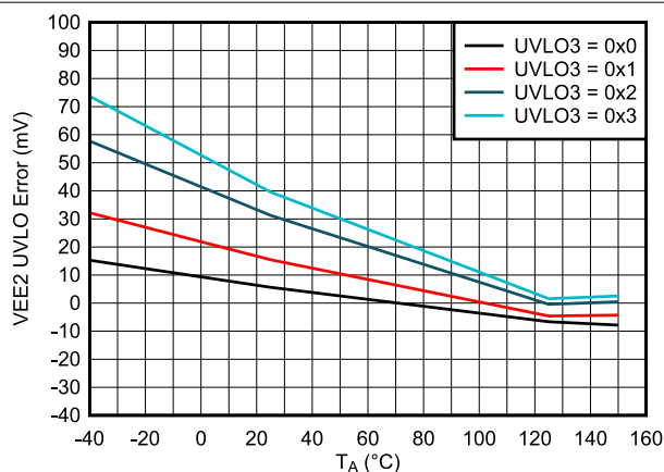
Figure 6-11. VEE2 UVLO Error vs. Temperature
