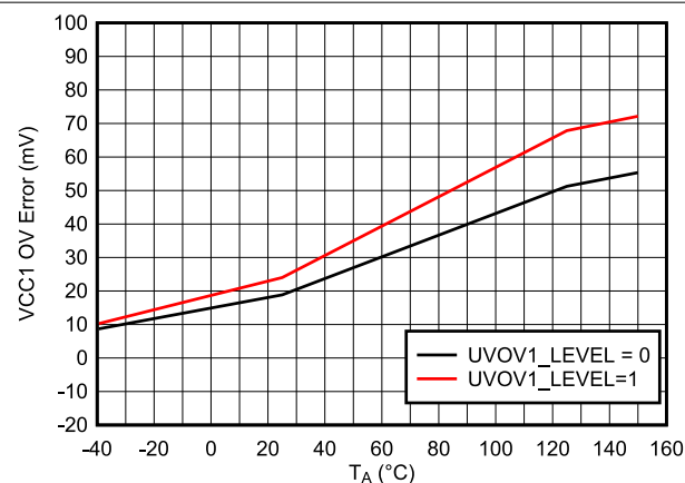
Figure 6-12. VCC1 OVLO Error vs. Temperature
