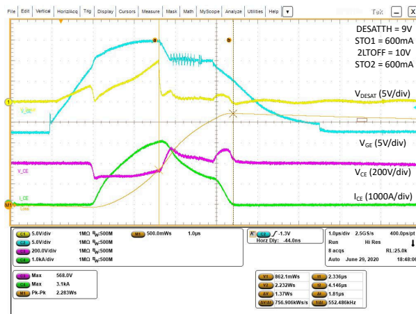
Figure 8-11. Two-Level Turn Off (2LTOFF) Shutdown Response to DESAT Event
