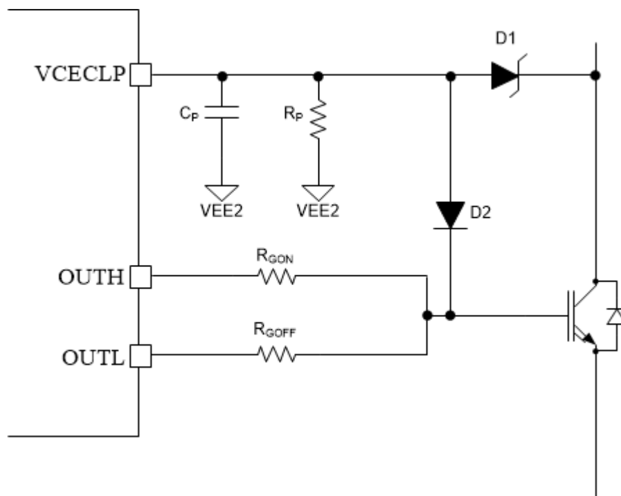
Figure 8-4. VCECLP External Components
