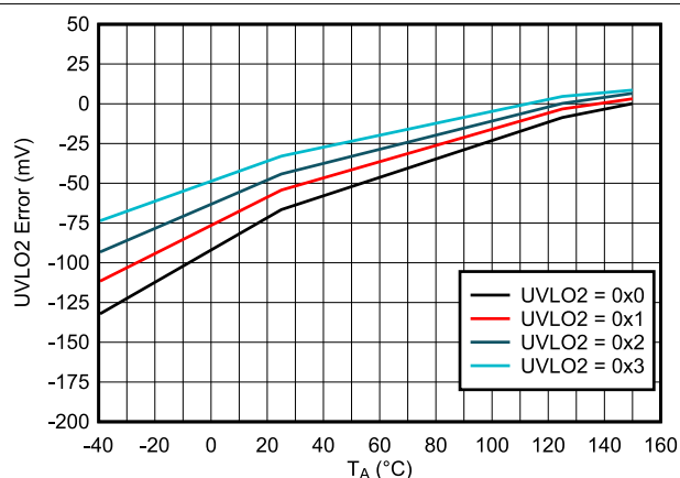
Figure 6-10. UVLO2 Error vs. Temperature
