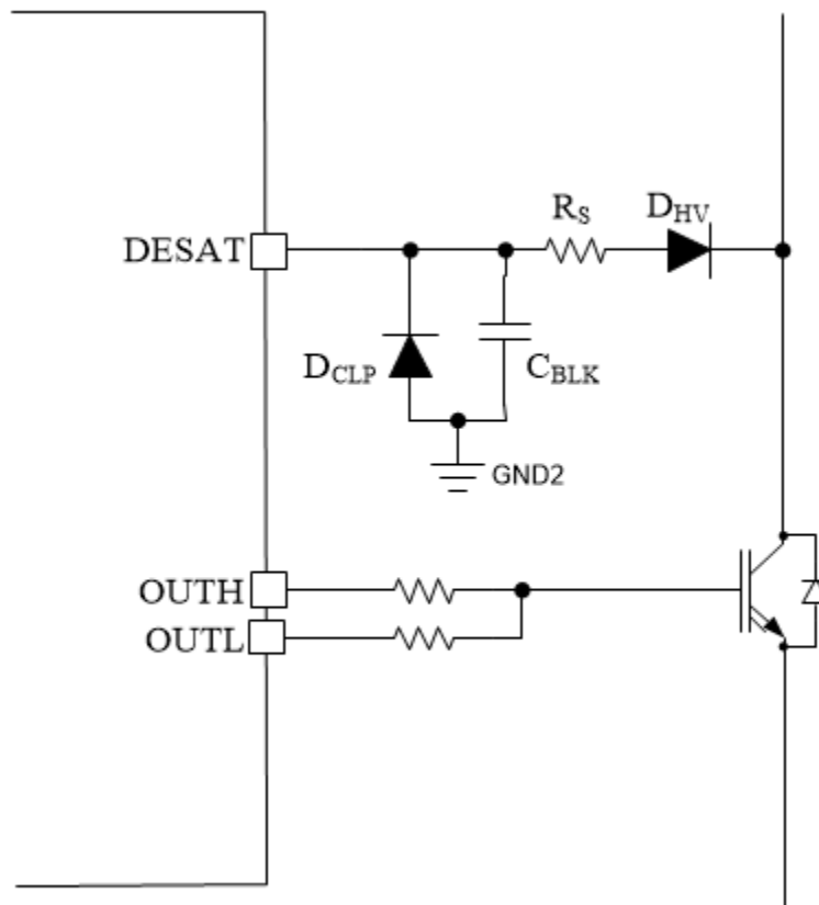
Figure 8-9. External Components for DESAT
