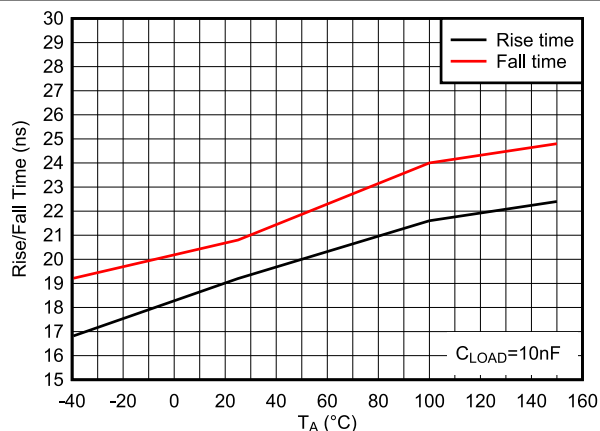
Figure 6-8. Rise/Fall Time vs. Temperature
