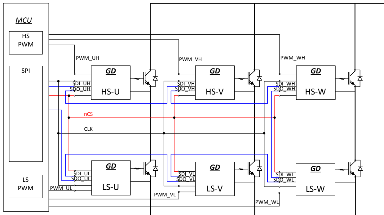
Figure 7-40. System configuration of daisy chain SPI configuration
