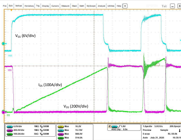
Figure 8-6. SiC Double Pulse Waveform
