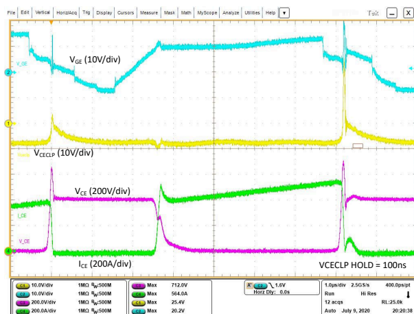
Figure 8-7. VCE Clamp Response with 100ns Hold Time
