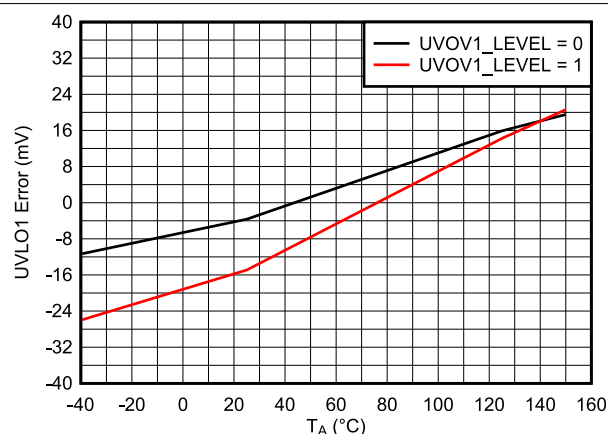
Figure 6-9. UVLO Threshold Error vs. Temperature
