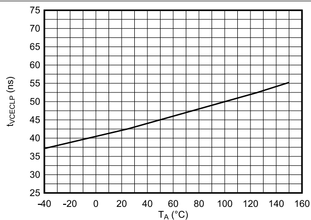
Figure 6-19. VCECLP Intervention Time vs. Temperature
