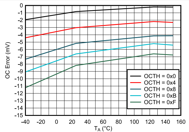
Figure 6-16. OC Threshold Error vs. Temperature
