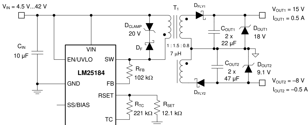
图 34. Schematic for Design 2 With V_{IN(nom)} = 24\text{ V} , V_{OUT1} = 15\text{ V} , V_{OUT2} = -8\text{ V} , I_{OUT} = 0.5\text{ A}
