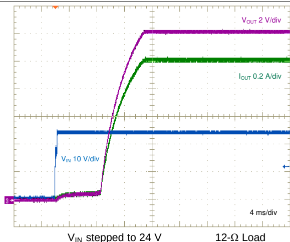
图 24. Start-up Characteristic
