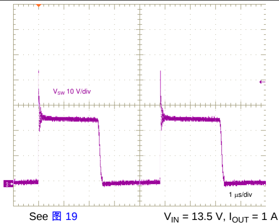
图 3. Switching Waveform in BCM
