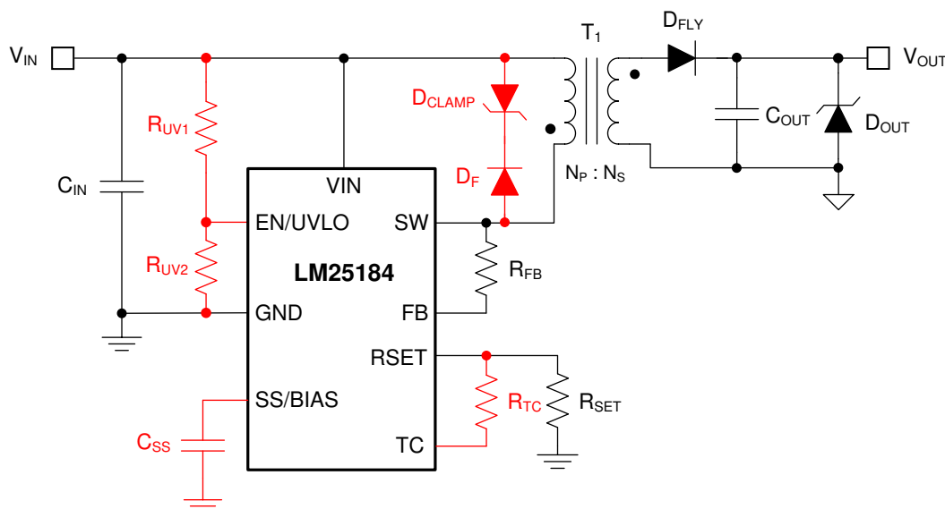
图 15. LM25184 Flyback Converter Schematic (Optional Components in Red)
