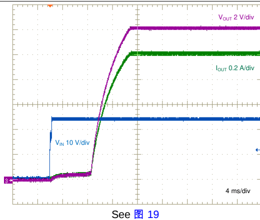
图 5. Start-up Characteristic
