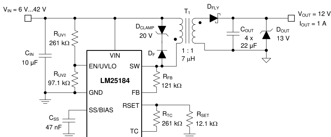
图 19. Schematic for Design 1 With V_{IN(nom)} = 24\text{ V} , V_{OUT} = 12\text{ V} , I_{OUT} = 1\text{ A}
