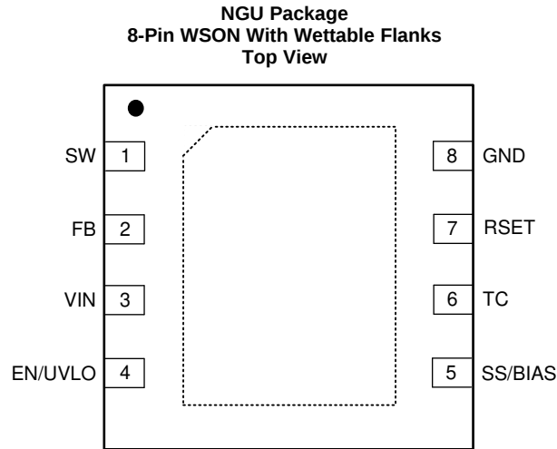
Pin Functions
