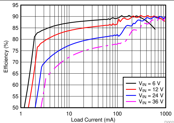
图 21. Efficiency (Log Scale)
