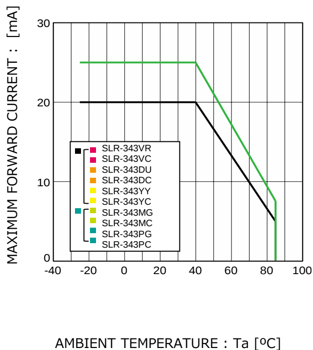
Fig.4 Derating
