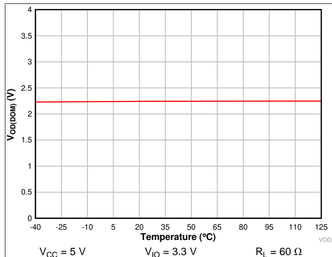
图 1. V_{OD(DOM)} vs Temperature
