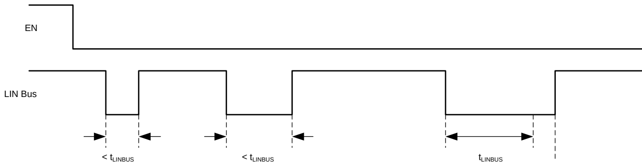
图 30. No Bus Fault: Entering Sleep Mode with Bus Recessive Condition and Wakeup
