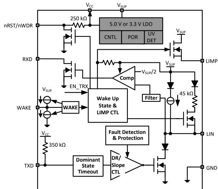
图 26. Transceiver plus VREG Functional Block Diagram
