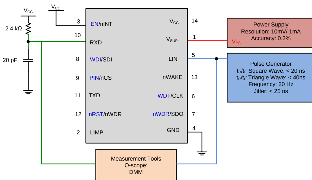
图 19. Propagation Delay Test Circuit
