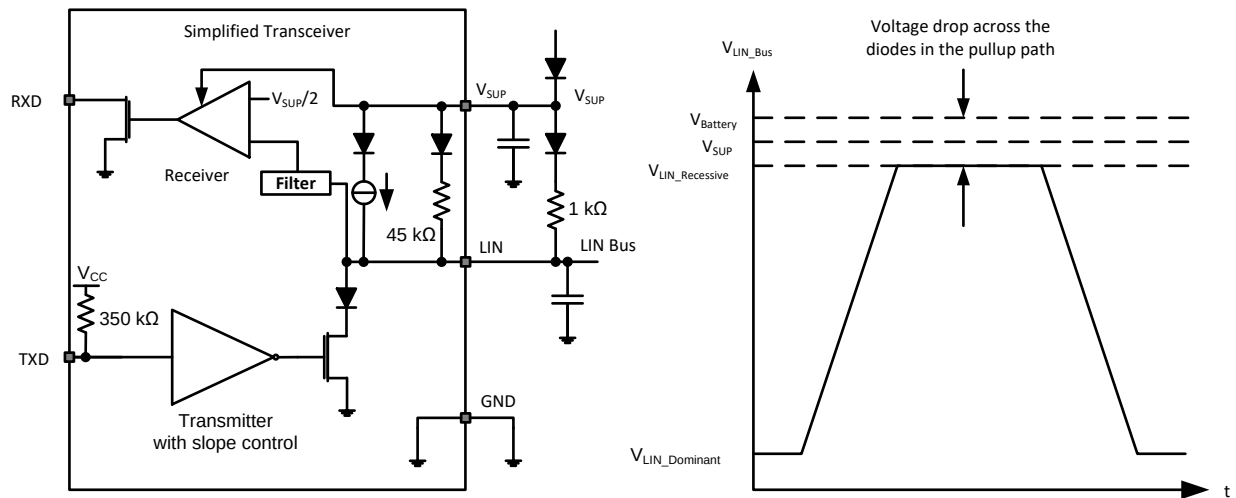
图 28. Master Node Configuration with Voltage Levels
