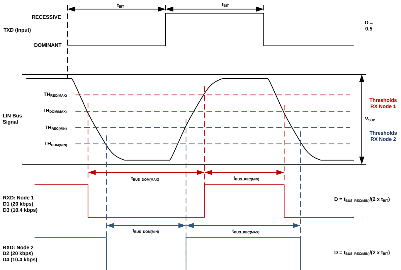
图 18. Definition of Bus Timing
