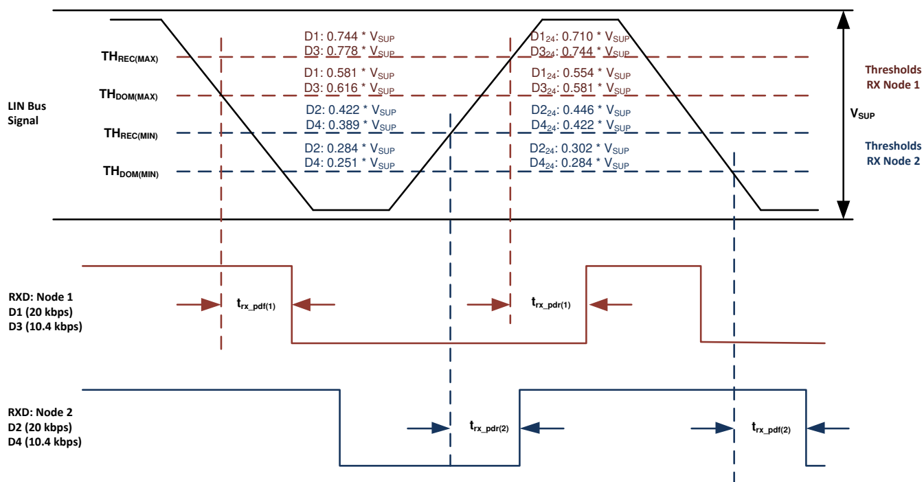
Figure 8-11. Propagation Delay
