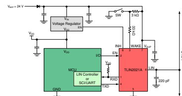
Simplified Responder Node Schematic (2)
