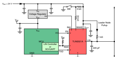
Simplified Commander Node Schematic (1)
